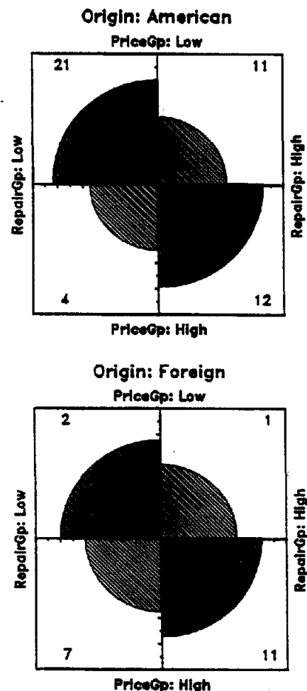
Figure 5: Fourfold display of automobiles
