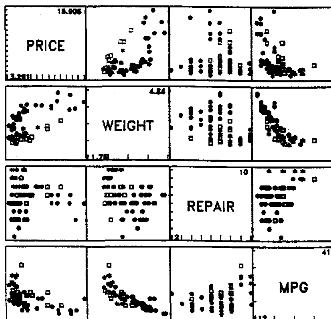
Figure 3: Scatterplot matrix for AUTO data. US models: circles, European: squares, Japanese: stars.
