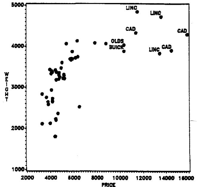
Figure 1: Plot of automobile data with extreme points labelled
