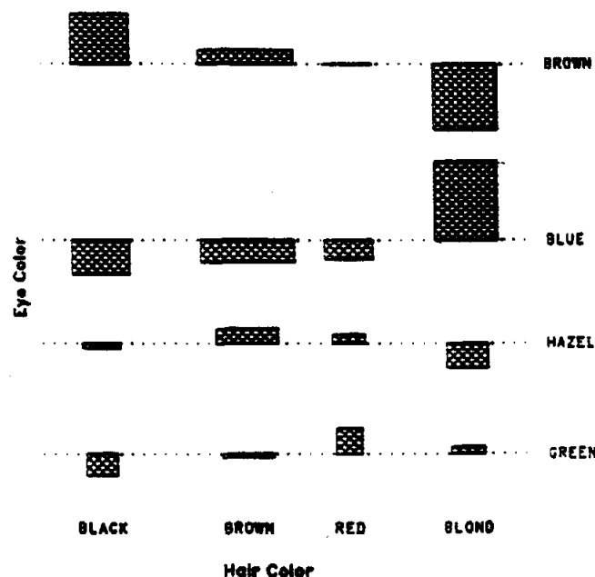
Figure 3: Association plot for hair-eye data
