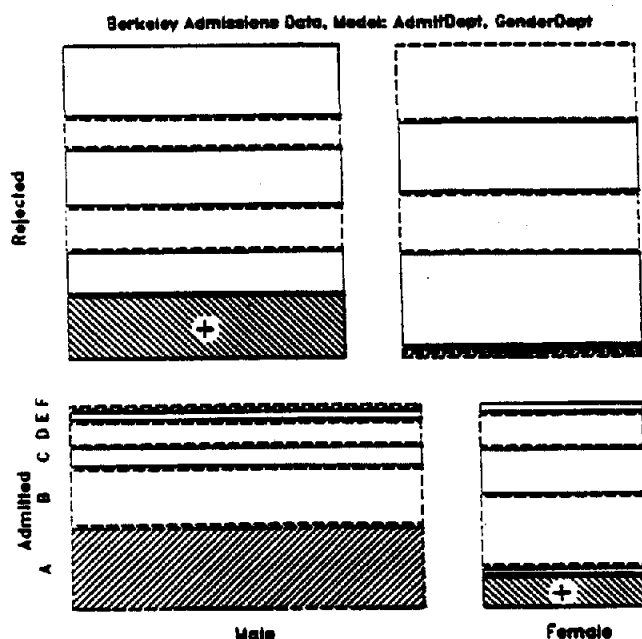
Figure 10: Mosaic display of Berkeley admissions data
