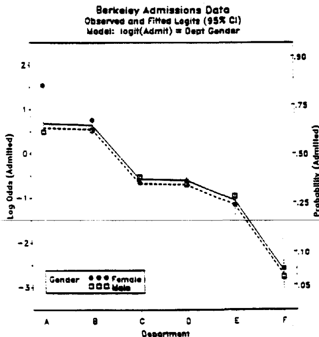
Figure 9: Effects of Gender and Department on Admission
