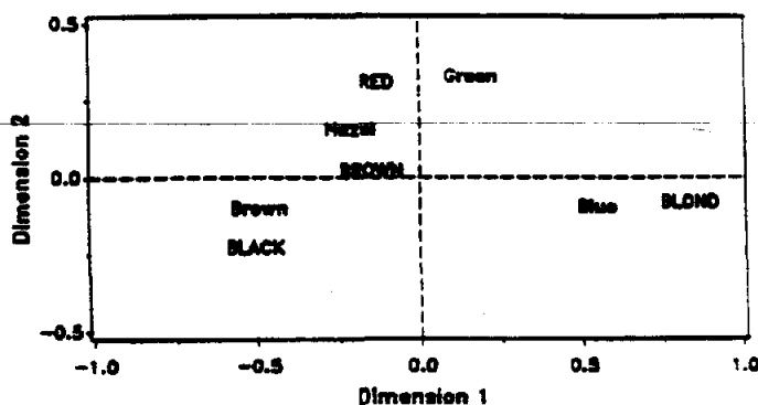
Figure 8: Correspondence analysis plot
