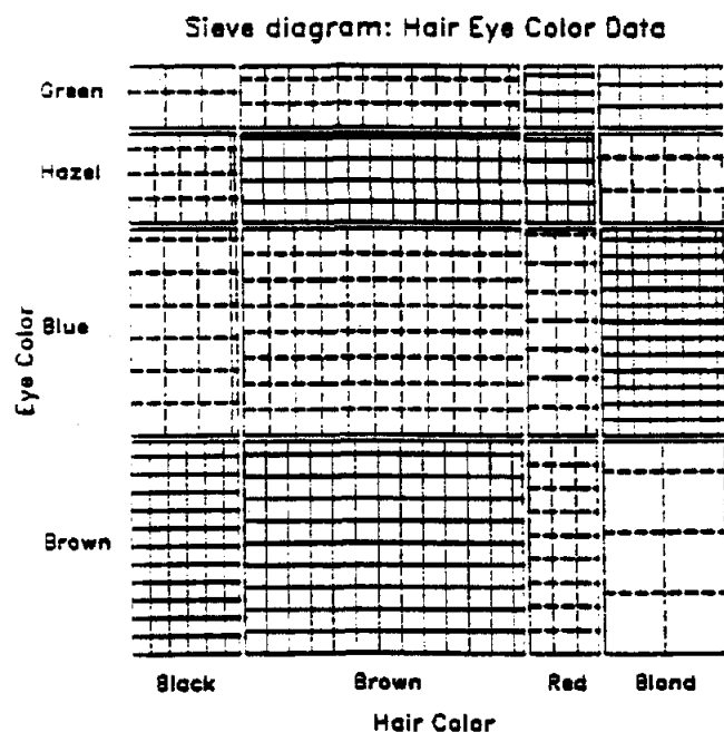
Figure 2: Sieve diagram for hair-eye data
