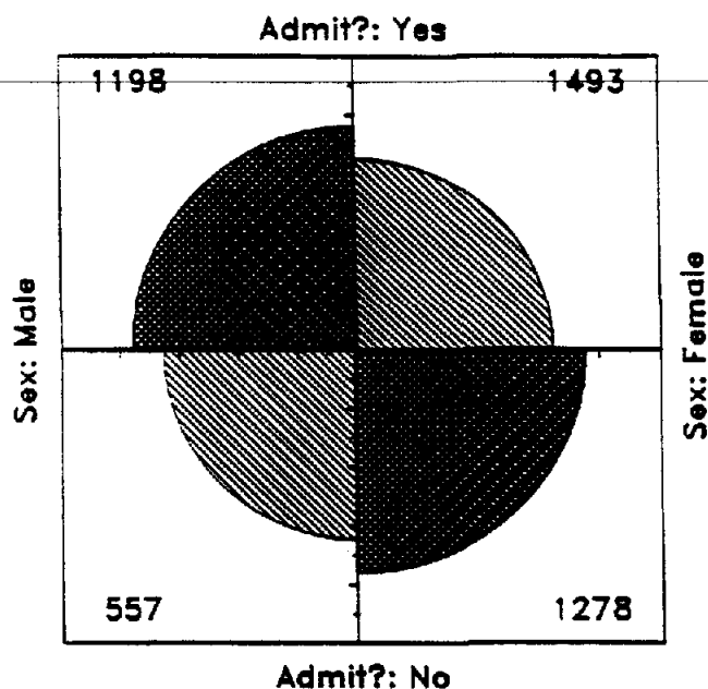
Figure 4: Four-fold display for Berkeley admissions
