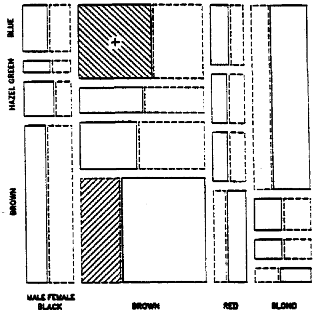
Figure 7: Mosaic display for hair color, eye color, and sex
