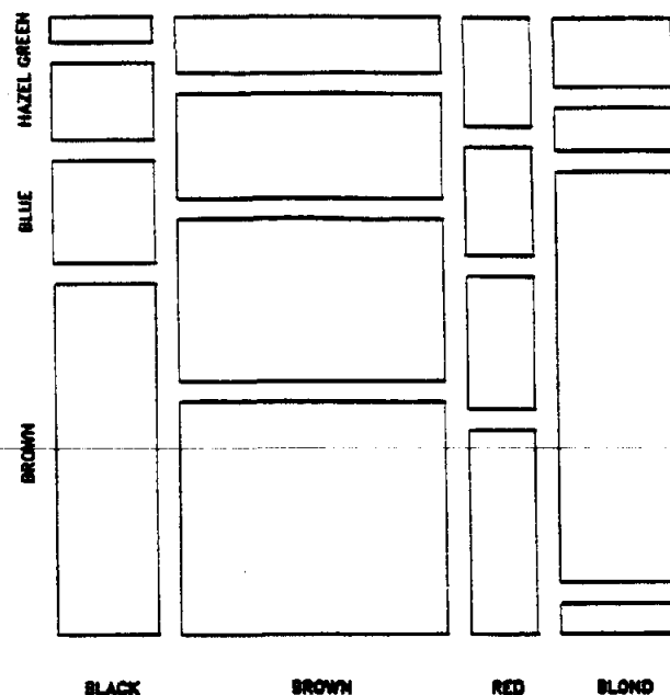
Figure 5: Condensed column proportion mosaic
