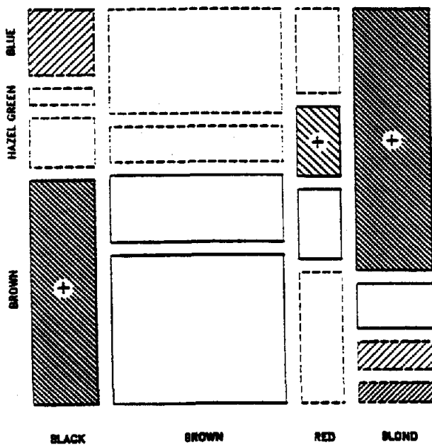
Figure 6: Enhanced mosaic, reordered and shaded
