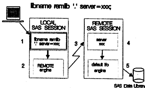
Figure 5 LIBNAME Statement for Remote Data Library
