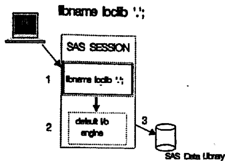
Figure 4 LIBNAME Statement for Local Data Library
