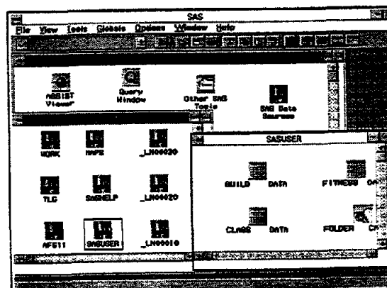
Figure 8: SAS/ASSIST Desktop
