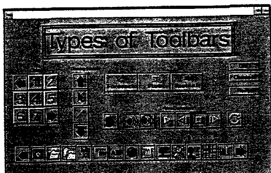
Figure 7: Toolbar Objects
