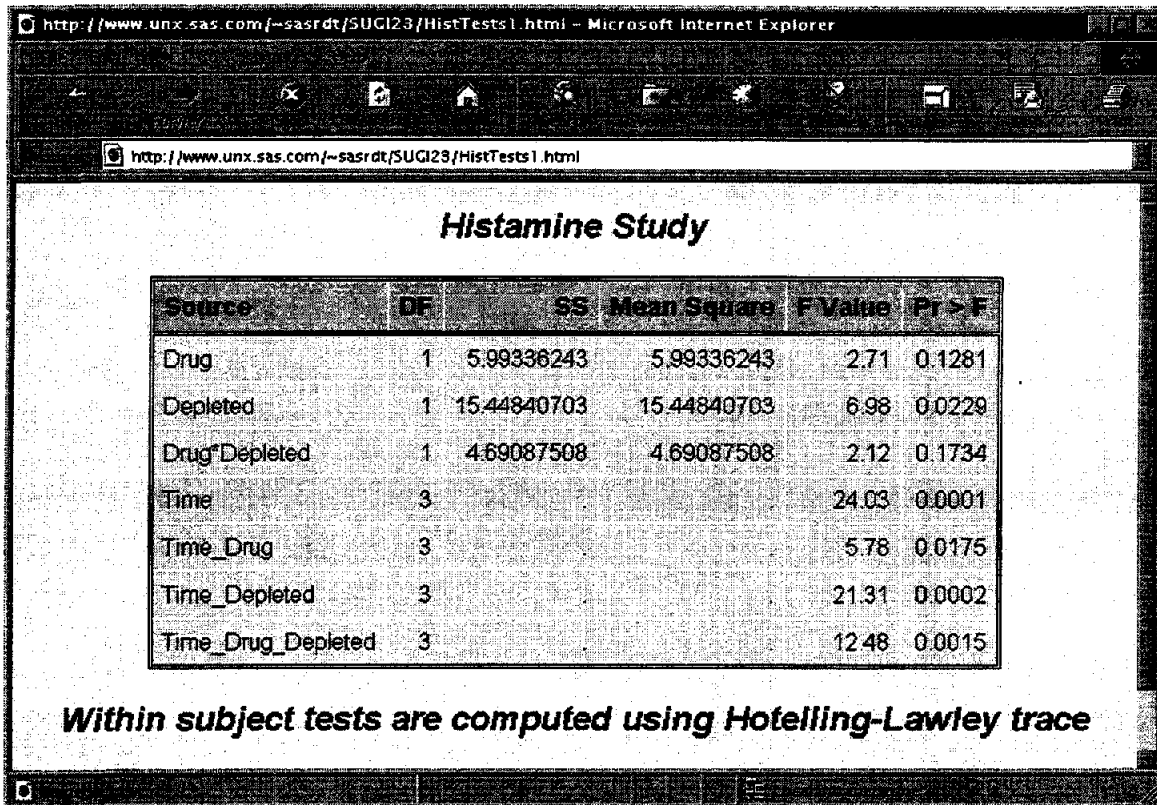
Figure 9: Combined tests for within- and between-subject effects
