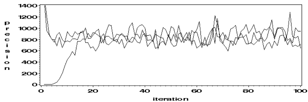
Figure 3: chainplots for two parameters
