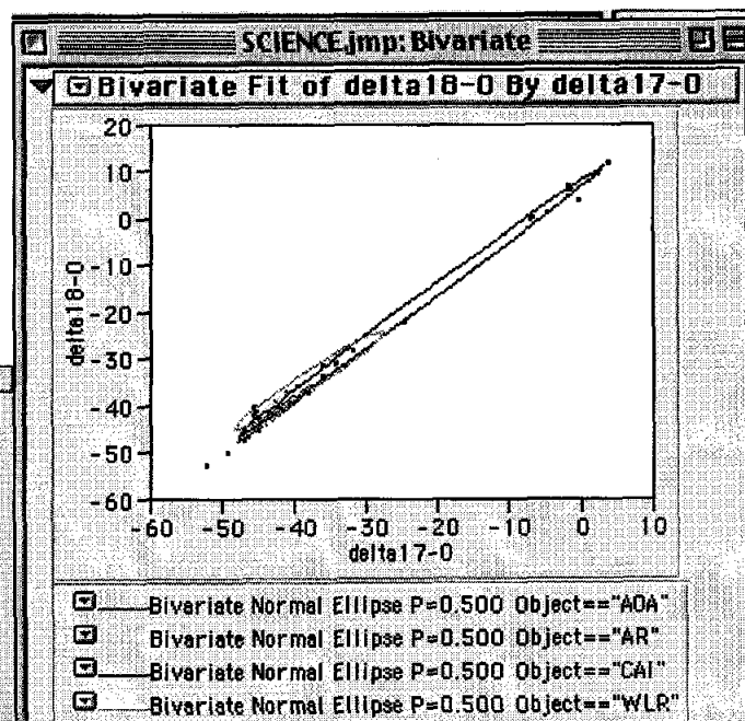
Fig. W3: Correlation Analysis
