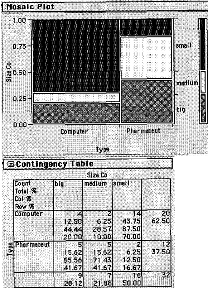
Fig. 4a1: Mosaic Plot with Contingency Table
