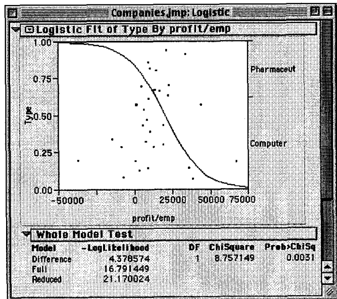
Fig. 4a3: Logistic Fit Analysis
