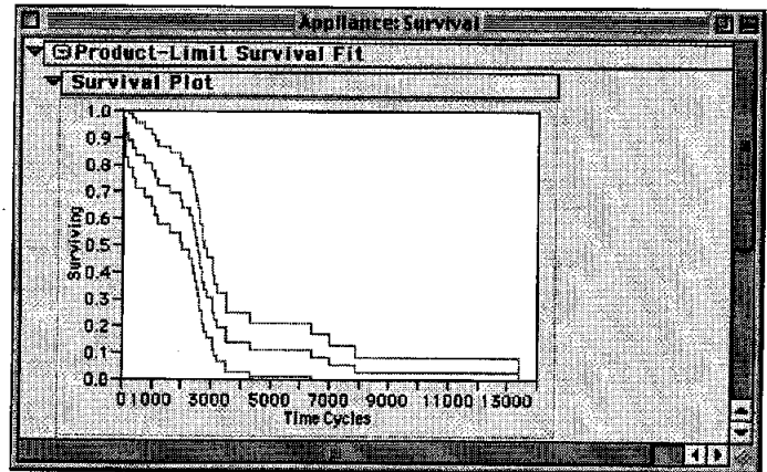
Fig. 4b2: Survivability / Reliability
