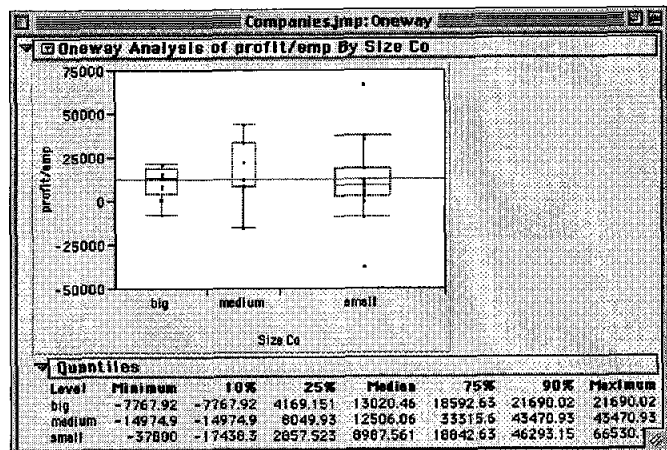
Fig. 4a2: One-Way Analysis of Variance
