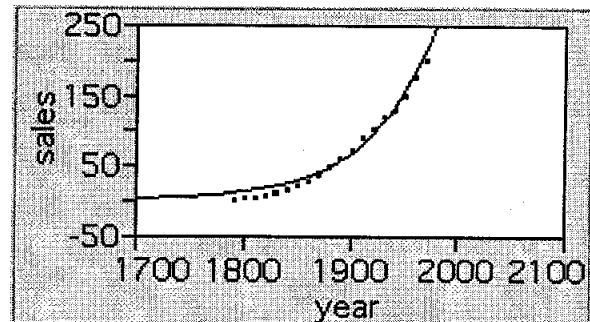
Fig. 4b3: Non-Linear XY-Fit
