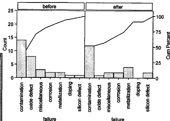
Fig. 3a/b: Pareto & Shewhart Control Charts
