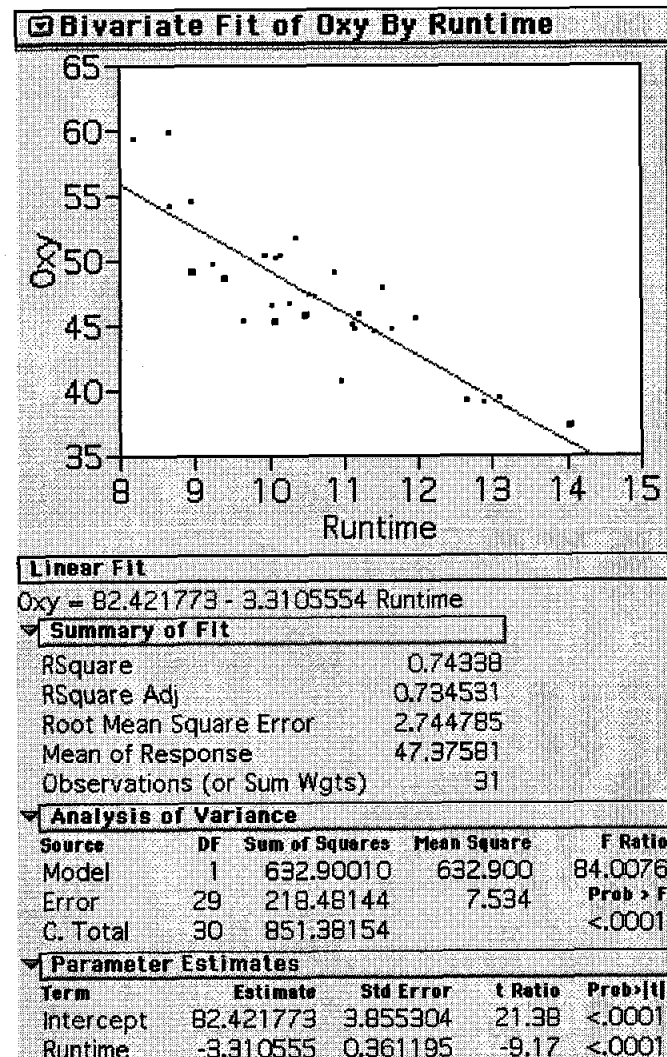
Fig. 4a4: XY-Fit Graph & Table
