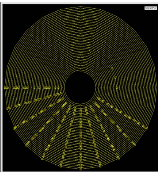
Figure 40: Time Spiral Plot of Sparse Data
