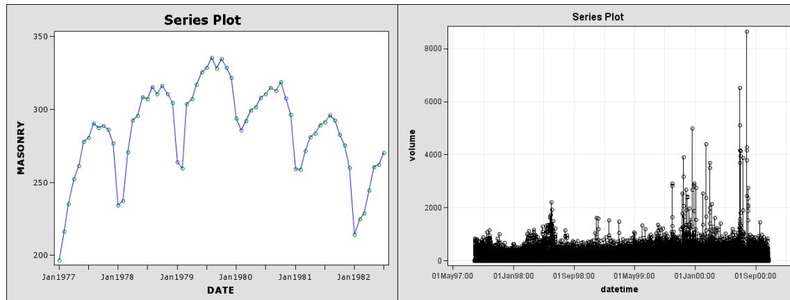
Figure 30: Monthly Observations
