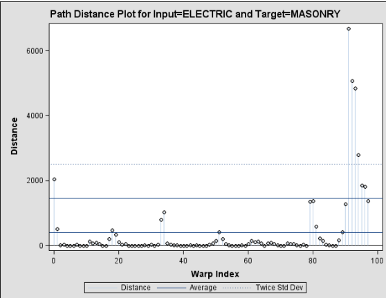
Figure 29: Path Distances
