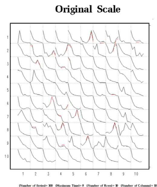
Figure 36: Longitudinal Plot
