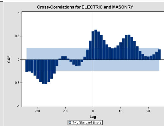
Figure 22: Cross-Correlations
