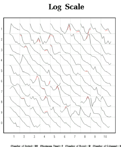
Figure 37: Log Transformed Longitudinal Plot
