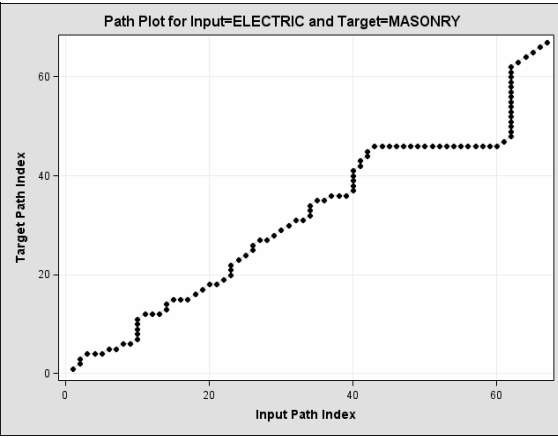
Figure 27: Warping Path
