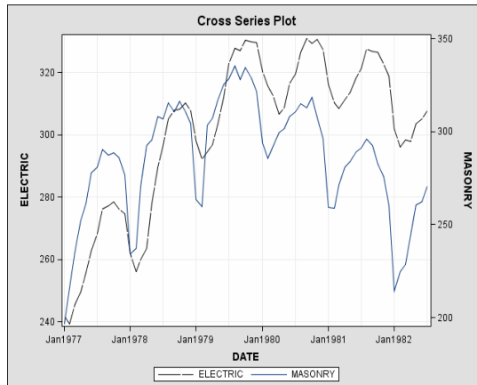
Figure 21: Cross Series
