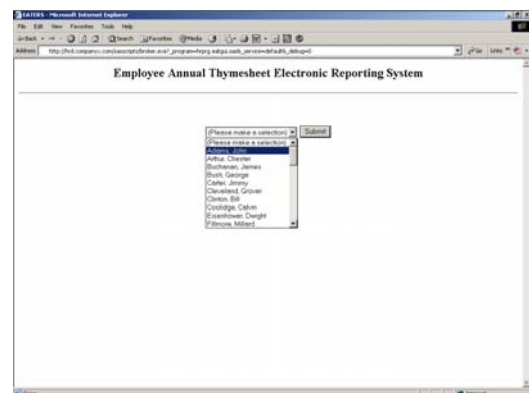
Figure 12. Modified GUI using a SAS program to dynamically generate the same HTML code that had been applied in the original eatgui.html document
