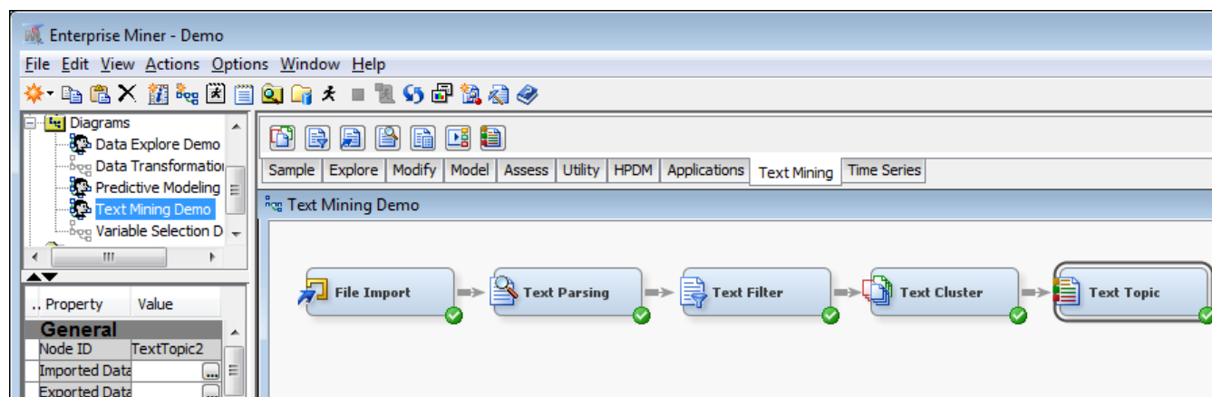
Figure 8. A Text Mining Procedure Example in SAS Enterprise Miner
