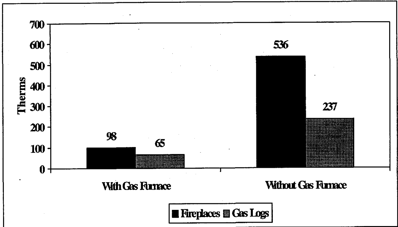
Chart 3. Weather Normalized Annual Gas Usage
