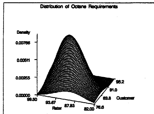
Figure 3. Surface of Density Estimate for BWM=2,2
