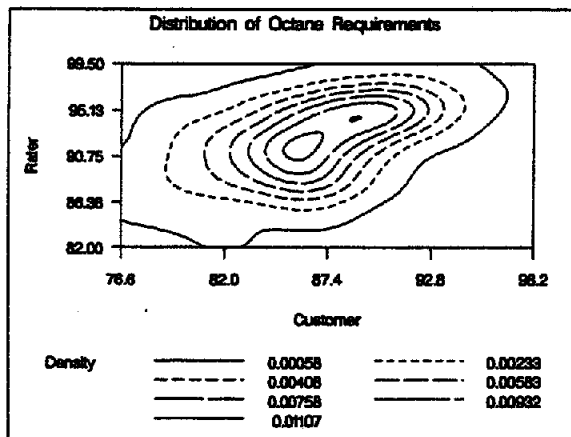
Figure 2. Contours of Density Estimate
