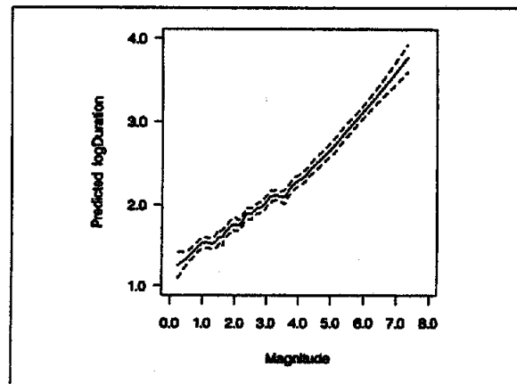
Figure 6. Loess Fit for Earthquake Data
