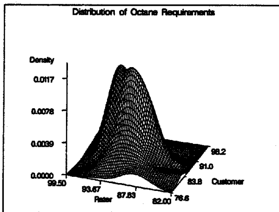
Figure 1. Surface of Density Estimate
