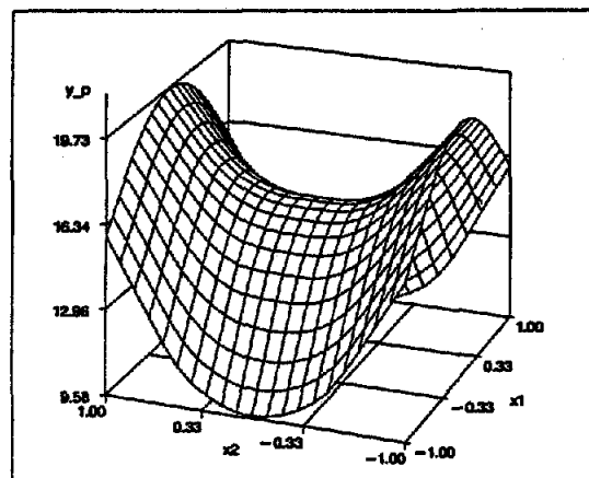
Figure 14. Fitted Surface Using Values in PRED.Y
