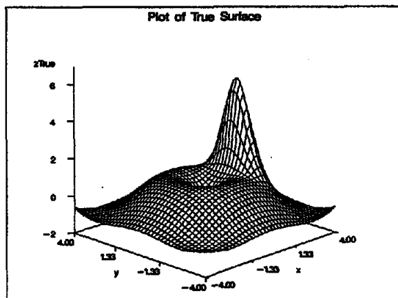
Figure 8. Plot of True Surface
