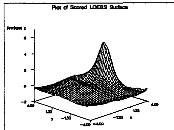
Figure 9. Plot of Scored LOESS Surface
