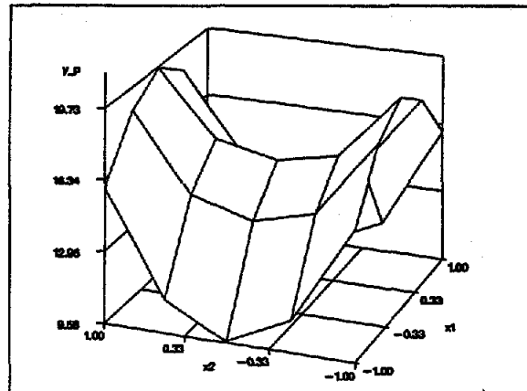
Figure 13. Fitted Surface Using Values in ESTIMATE
