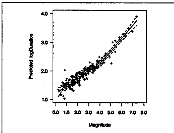
Figure 5. Loess Fit for Earthquake Data
