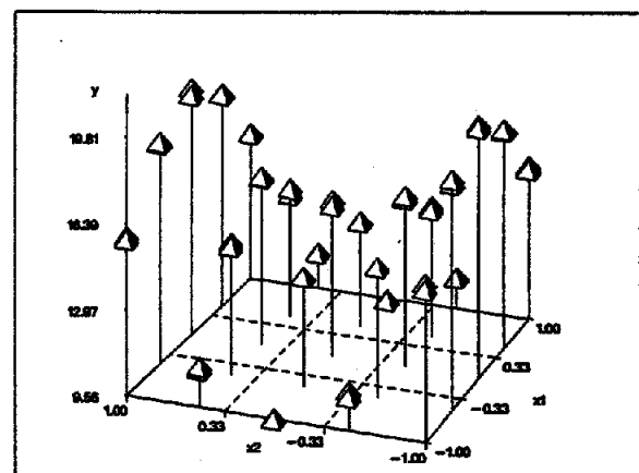
Figure 10. Plot of Data Set MEASURE
