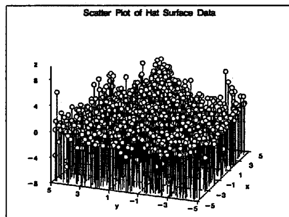
Figure 7. Scatter Plot of Cowboy Hat Surface Data
