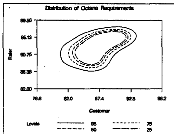
Figure 4. Level Contours for BMW=2,2
