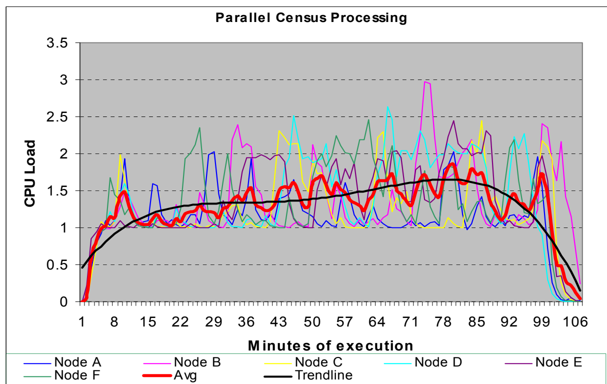
Figure 13. Execution in Parallel across Six Blade Server Nodes
