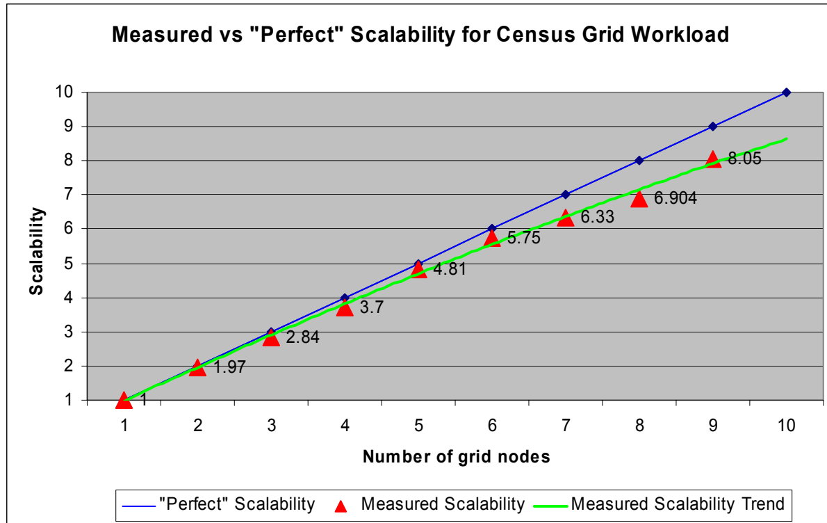
Figure 15. Measured Scalability for ThisTest Versus "Perfect" Scalability
