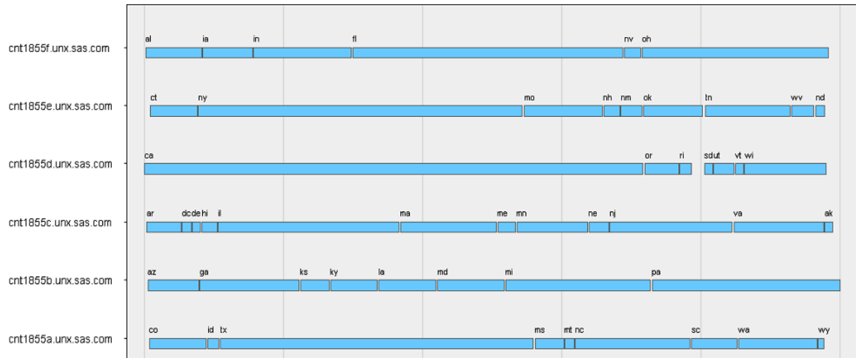
Figure 16. Census Workload Executed on Six Grid Nodes. SAS Data Integration Studio was configured to allow six jobs to run at a time. Grid nodes are along the Y axis, and elapsed time across the X axis.
