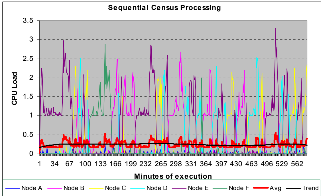
Figure 11. Elapsed Run Time Required for Sequential Execution of the Census Workload
