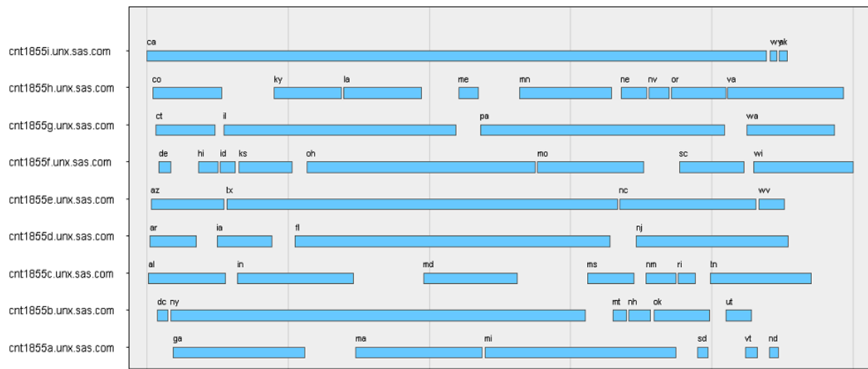
Figure 17. Census Workload Running across Nine Grid Nodes. SAS Data Integration Studio allowed eight workload elements to run at a time.
