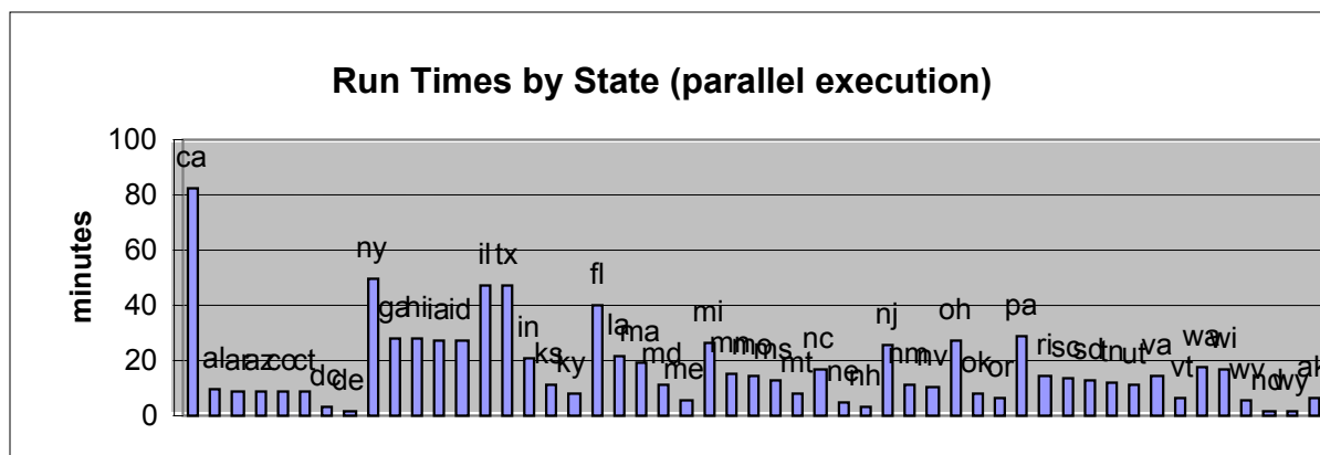
Figure 14. Execution Profile for Each Workload Element
