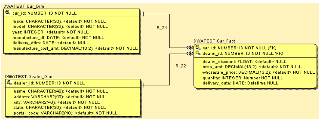
Figure 18. A Small Data Model. This diagram shows how three tables are related.
