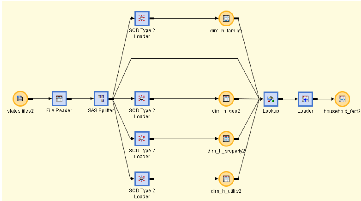
Figure 8. A Basic Process Flow That Builds a Star Schema of Four Dimensions and a Fact Table
