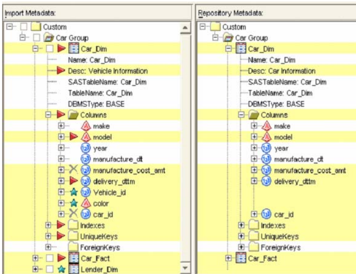
Figure 20. Metadata Difference View
