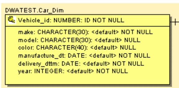
Figure 19. An Updated Version of the Car_Dim Table Structure. Various aspects of the table have been modified.
