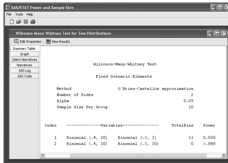
Figure 35. Wilcoxon Results
