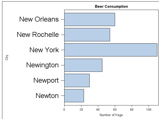
Figure 3: Binary Collation
