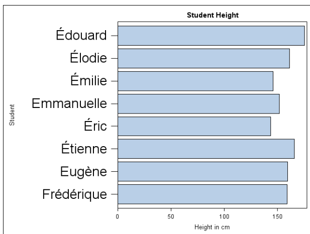
Figure 2: Linguistic Collation
