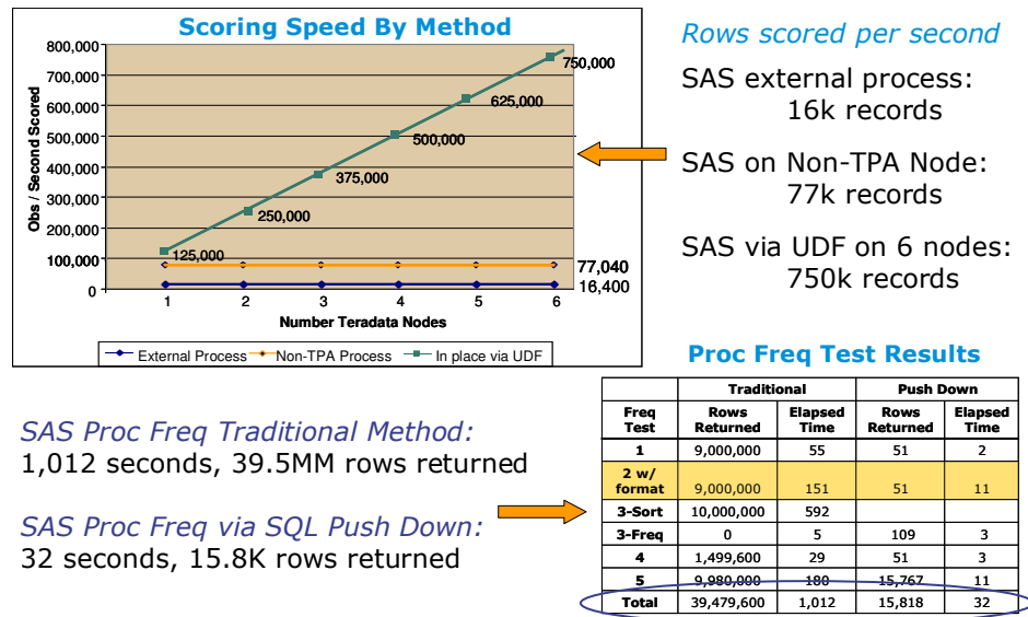
Figure 3: Benchmarking Results
