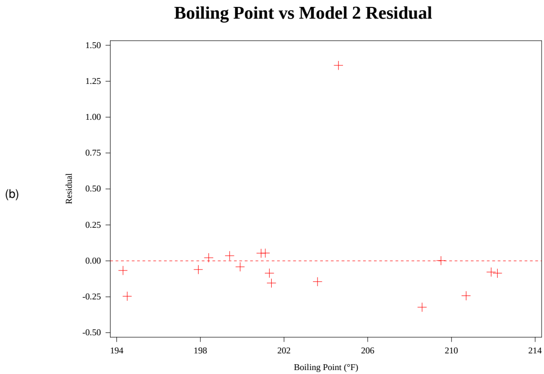
Figure 3: Scatterplot and regression line (a) and residual plot (b) of model 2 of Forbes' Data, originally from Forbes (1857) and described in detail in Weisberg (2005, pp. 4-6).
