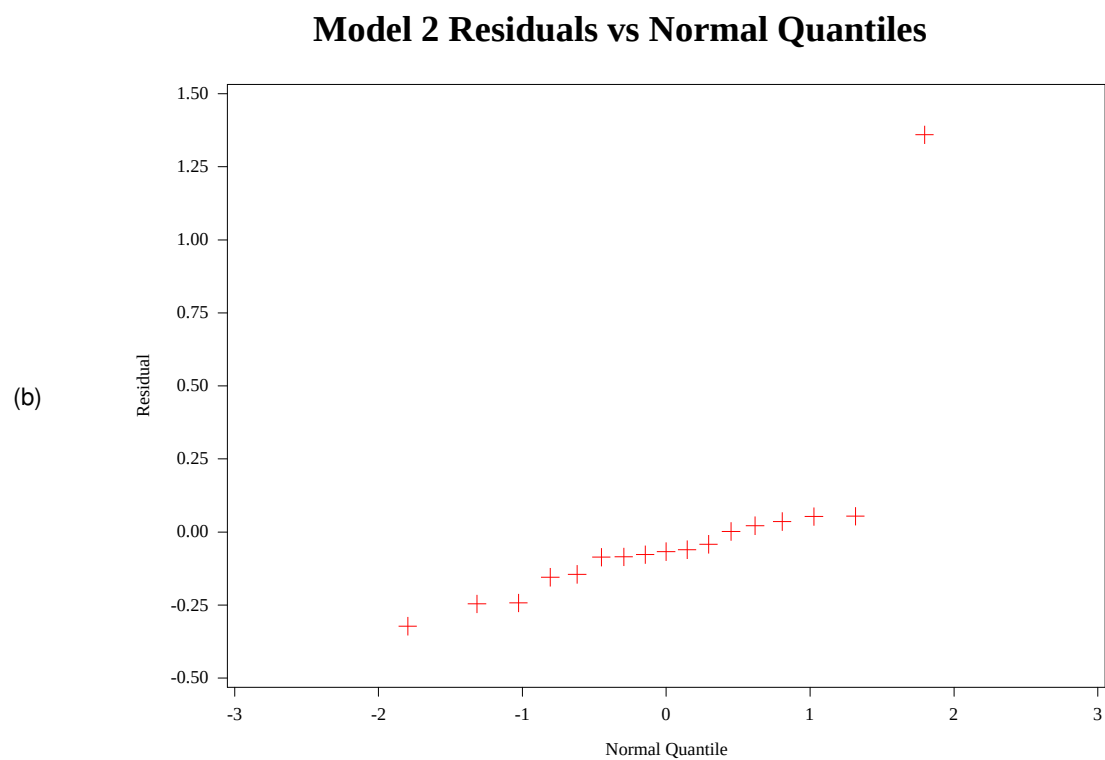
Figure 4: Q-Q Plots for model 1 (a: boiling point vs pressure) and model 2 (b: boiling point vs log pressure) of Forbes' data.
