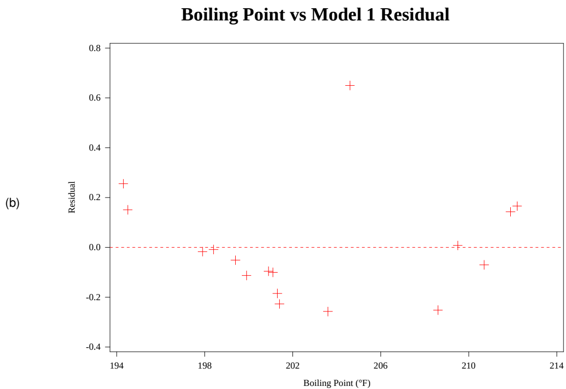
Figure 2: Scatterplot and regression line (a) and residual plot (b) of Forbes' Data, originally from Forbes (1857) and described in detail in Weisberg (2005, pp. 4-6).
