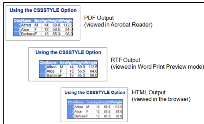
Figure 4: Output from Simple CSSSTYLE= Option Usage
