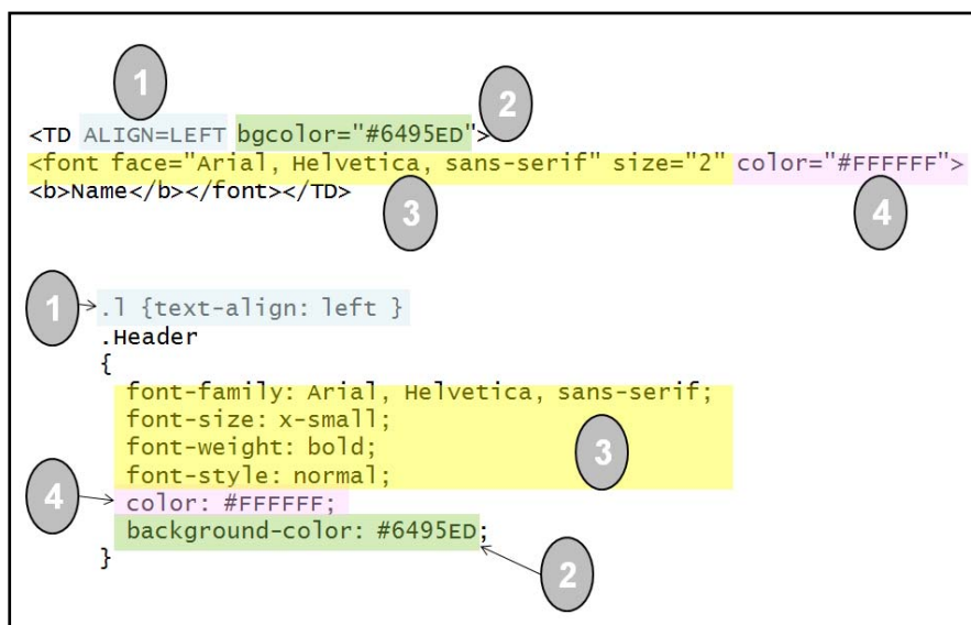
Figure 2: Comparison of Embedded Method with CSS Method of Specifying Style
