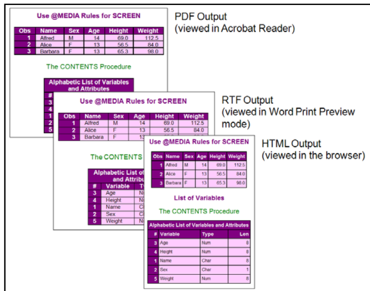
Figure 6: Using the SCREEN @MEDIA CSS Rule
