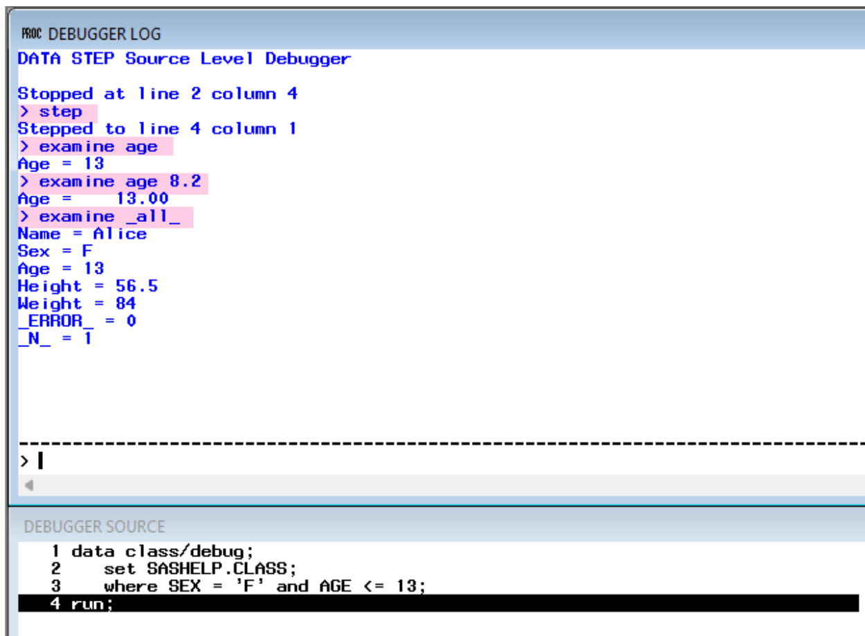
Image 2: Illustration of SAS Display Manager DATA Step Debugger
