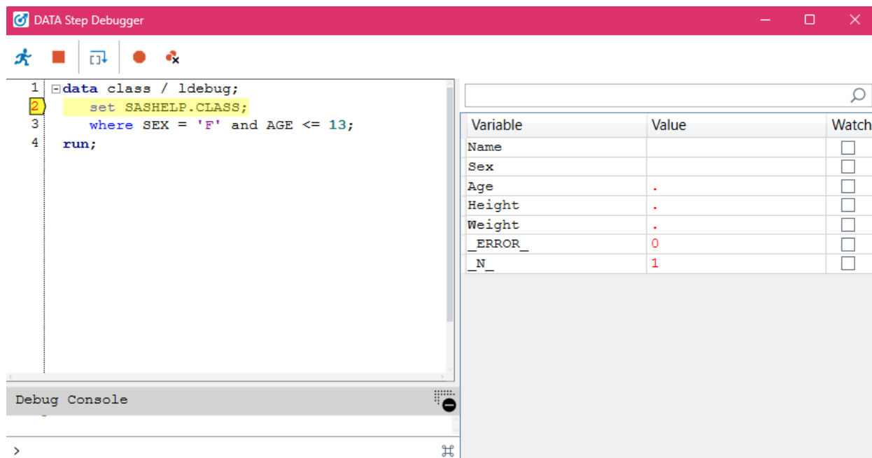
Image 4: SAS Enterprise Guide DATA Step Debugger Window
