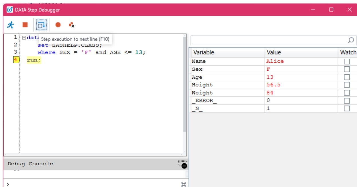
Image 5: Illustration of SAS Enterprise Guide DATA Step Debugger
