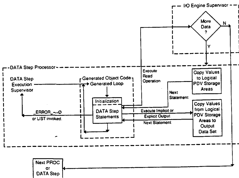
Figure 4 Execution Time Logic Flow
