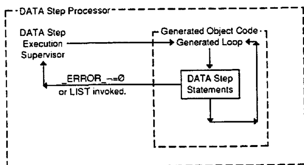
Figure 3 Compiler Generated DATA Step Loop
