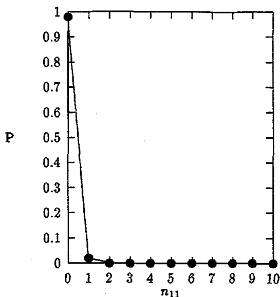
Figure 6: n_{++} = 10000 , n_{1+} = 20 , n_{+1} = 10
