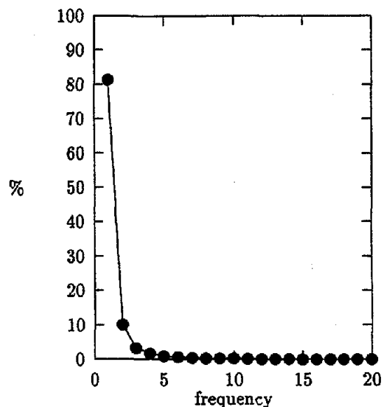
Figure 2: Distribution of bigrams
