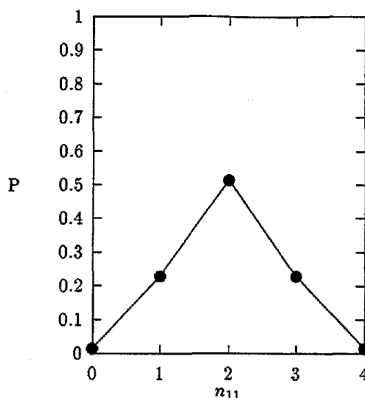
Figure 5: n_{++} = 8, n_{1+} = 4, n_{+1} = 4
