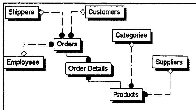
Figure 1. Main subject Area ERD
