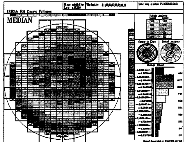
Figure 9 - Parameter Wafermap Analysis graph
