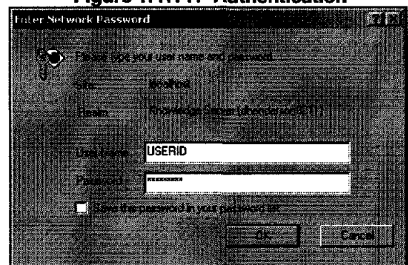
Figure 1. HTTP Authentication
