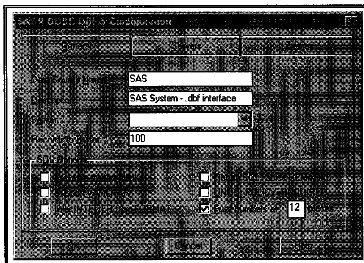
Figure "Q" - ODBC Driver Configuration - General Information
