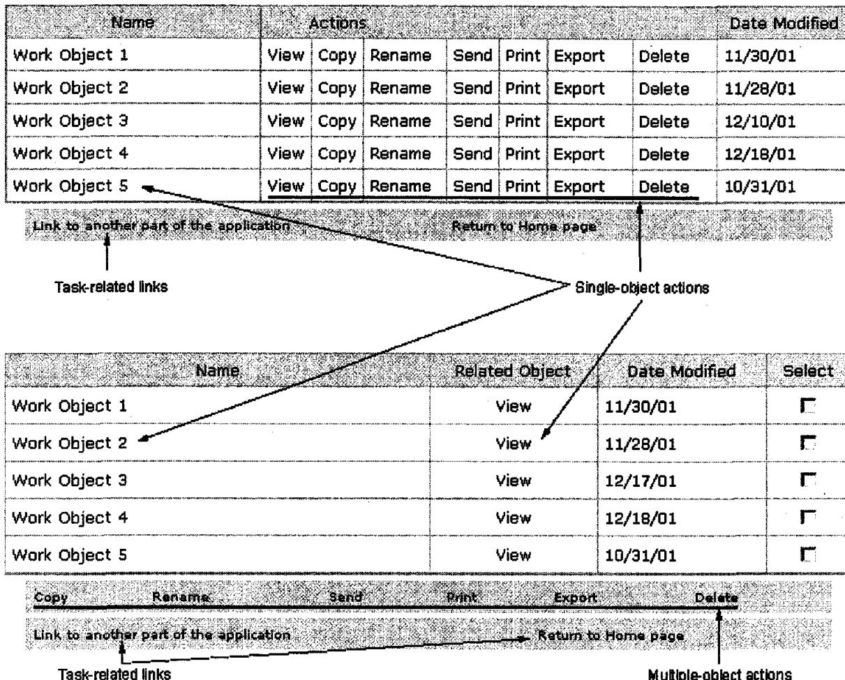
Figure 7. Alternative Table Designs
