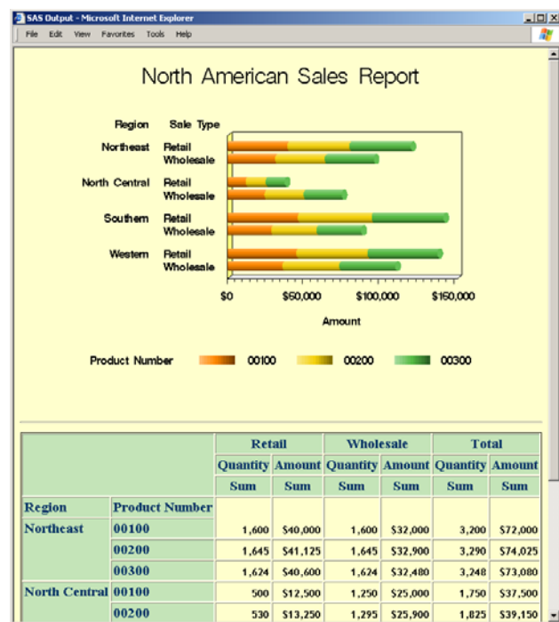
Figure 1. ODS-generated HTML output in a Web browser.
