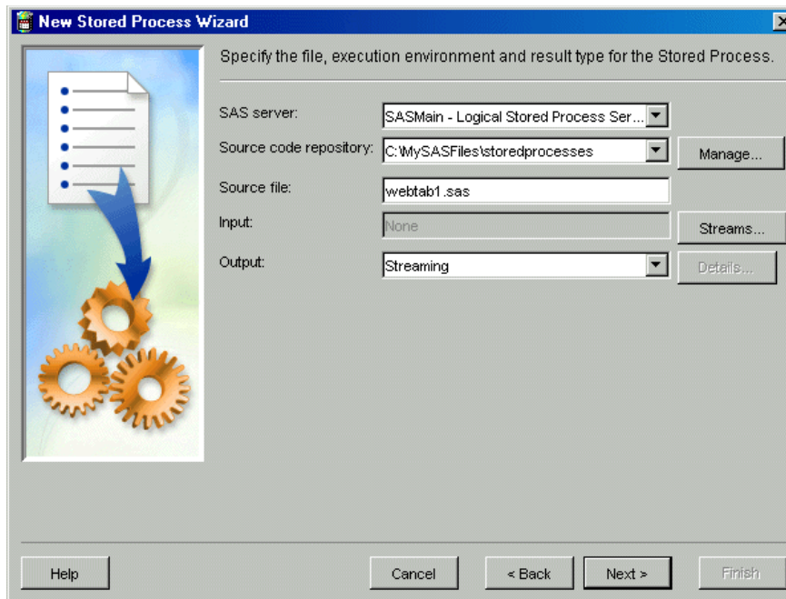
Figure 4. New Stored Process Wizard – Execution Details
