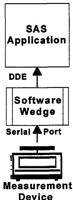
Figure 4 Using Third-Party Software
