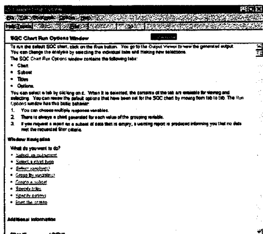
Figure 7 SQC Chart Run Options Window
