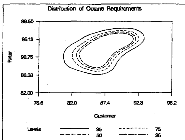
Figure 4. Level Contours for BMW=2,2
