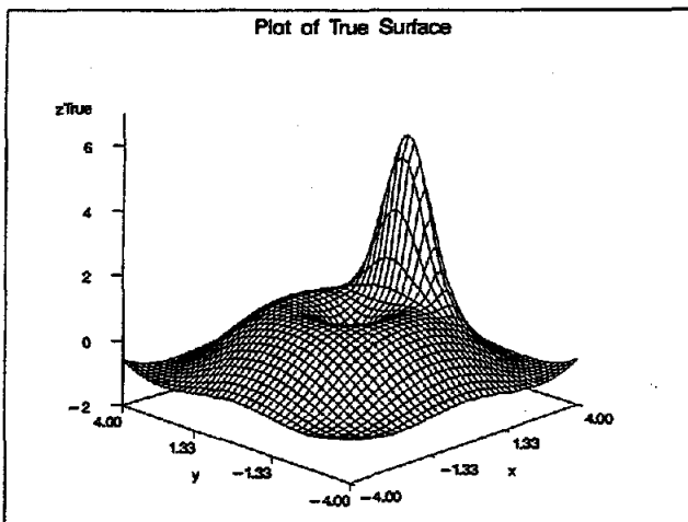
Figure 8. Plot of True Surface
