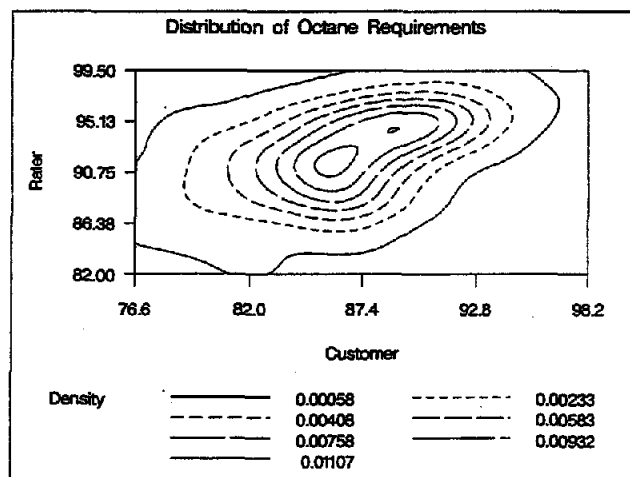
Figure 2. Contours of Density Estimate
