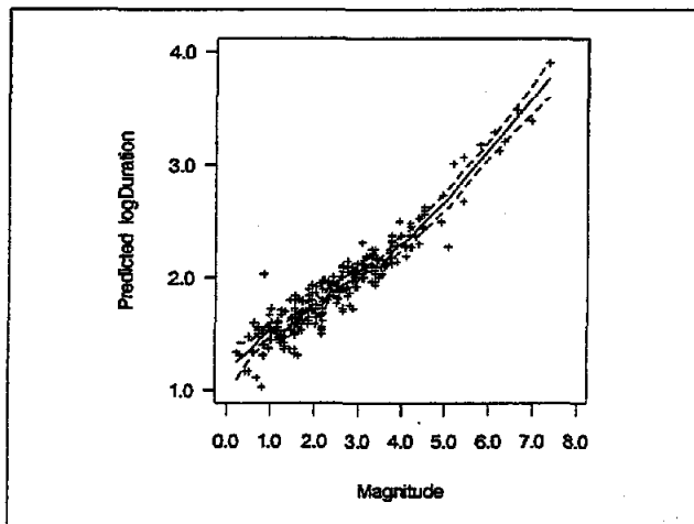
Figure 5. Loess Fit for Earthquake Data
