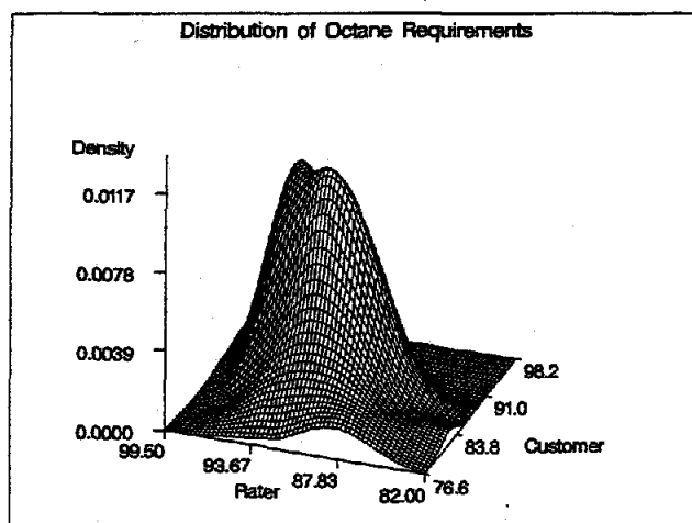
Figure 1. Surface of Density Estimate
