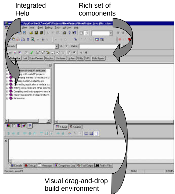
Figure 4. Initial webAF screen.
