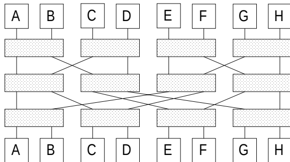
Figure 7: 2x2 Three-Stage Switched Network
