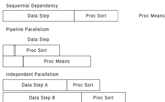
Figure 1. Types of Program Execution
