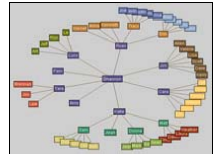
Treeview (DS2TREE)
