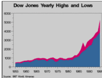
Area Plot
