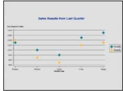
Scatter Plot
