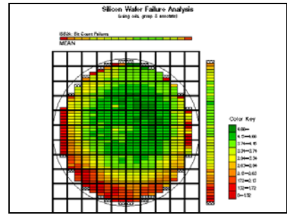
Wafer Map
