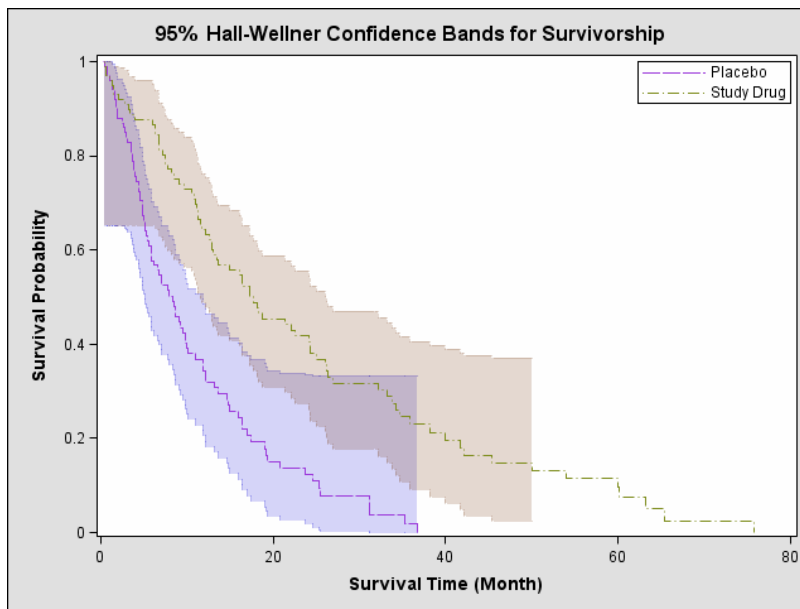
Figure 9. LIFETEST Procedure: Hall-Wellner Confidence Bands for Survival Functions
