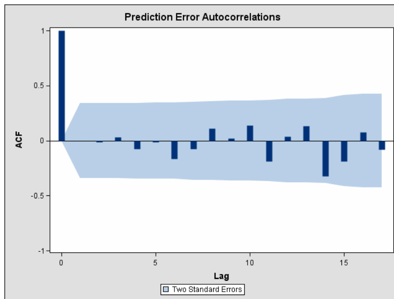
Figure 22. UCM Procedure: Prediction Error Autocorrelation Plot for Unobserved Component Model
