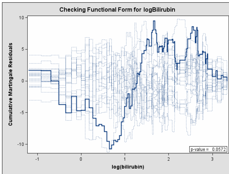
Figure 15. PHREG Procedure: Cumulative Residuals for Proportional Hazards Model
