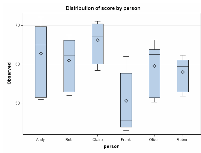
Figure 14. MIXED Procedure: Box Plot for Fixed Main Effects in Mixed Model
