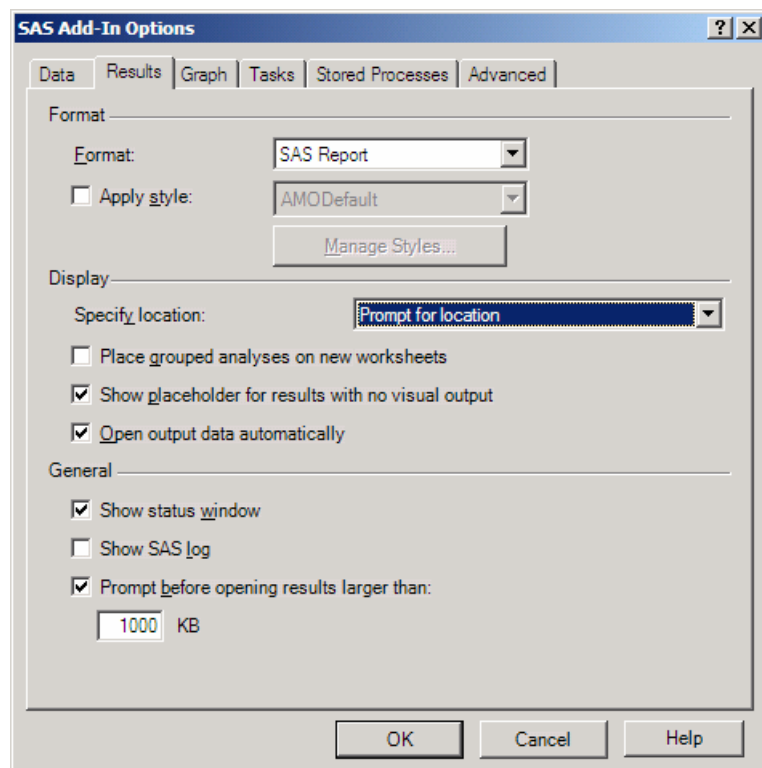
Figure 12. Results Tab in the SAS Add-In Options Dialog Box
