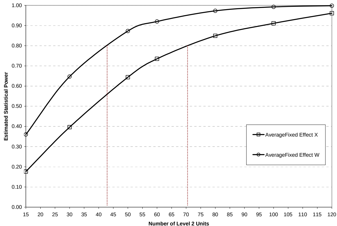
Figure 1. Estimated Statistical Power as a Function of the Number of Level 2 Units
