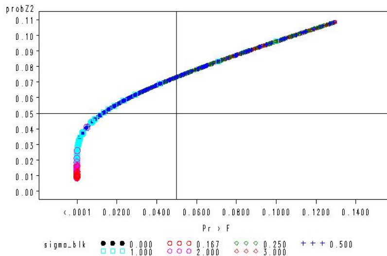
Figure 5: Wald p-values vs. F p-values
