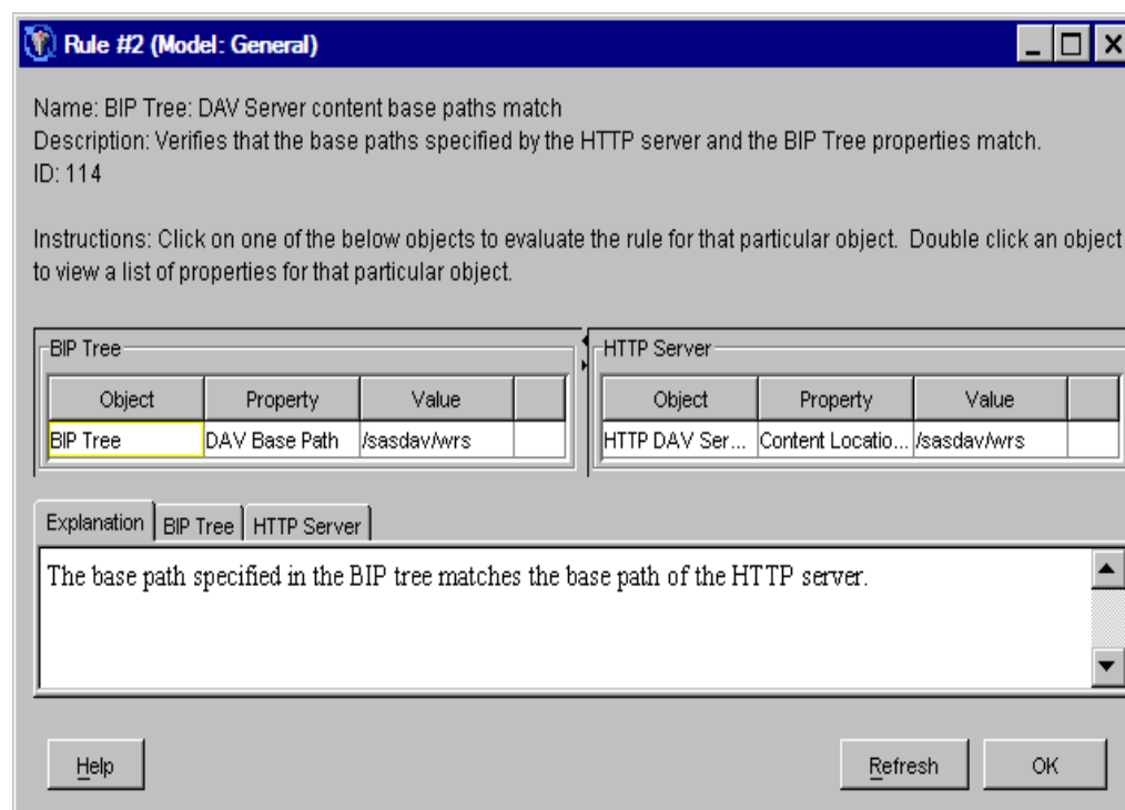
Display 17. Details of Rule 2
