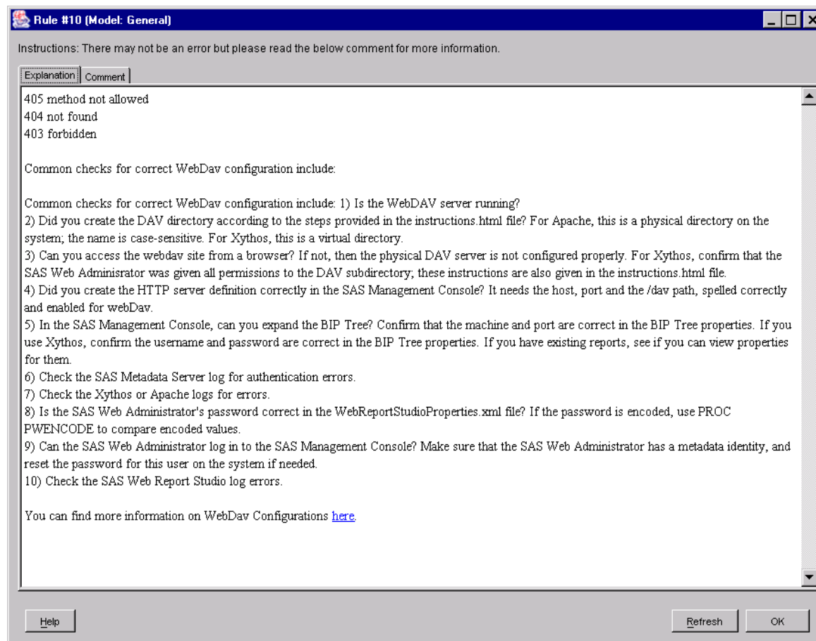
Display 3. WebDAV Informational Rule
