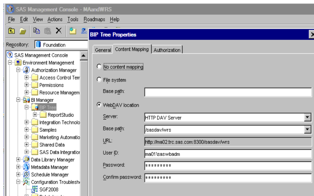
Display 18. Details of the Content Mapping Tab
