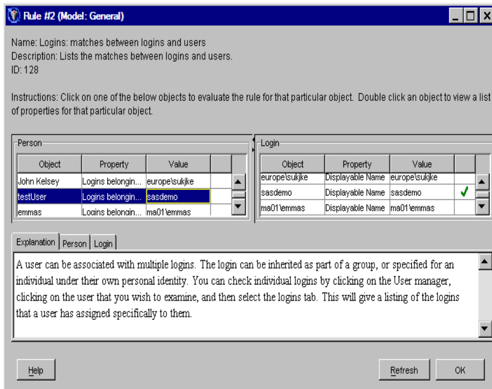
Display 11. Detailed Results from the Logins Rule
