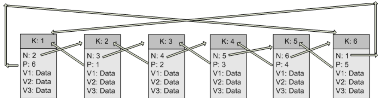
Illustration 5: Double Linked Circular list
