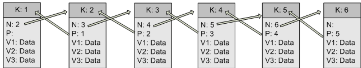
Illustration 3: Double Linked Linear List
