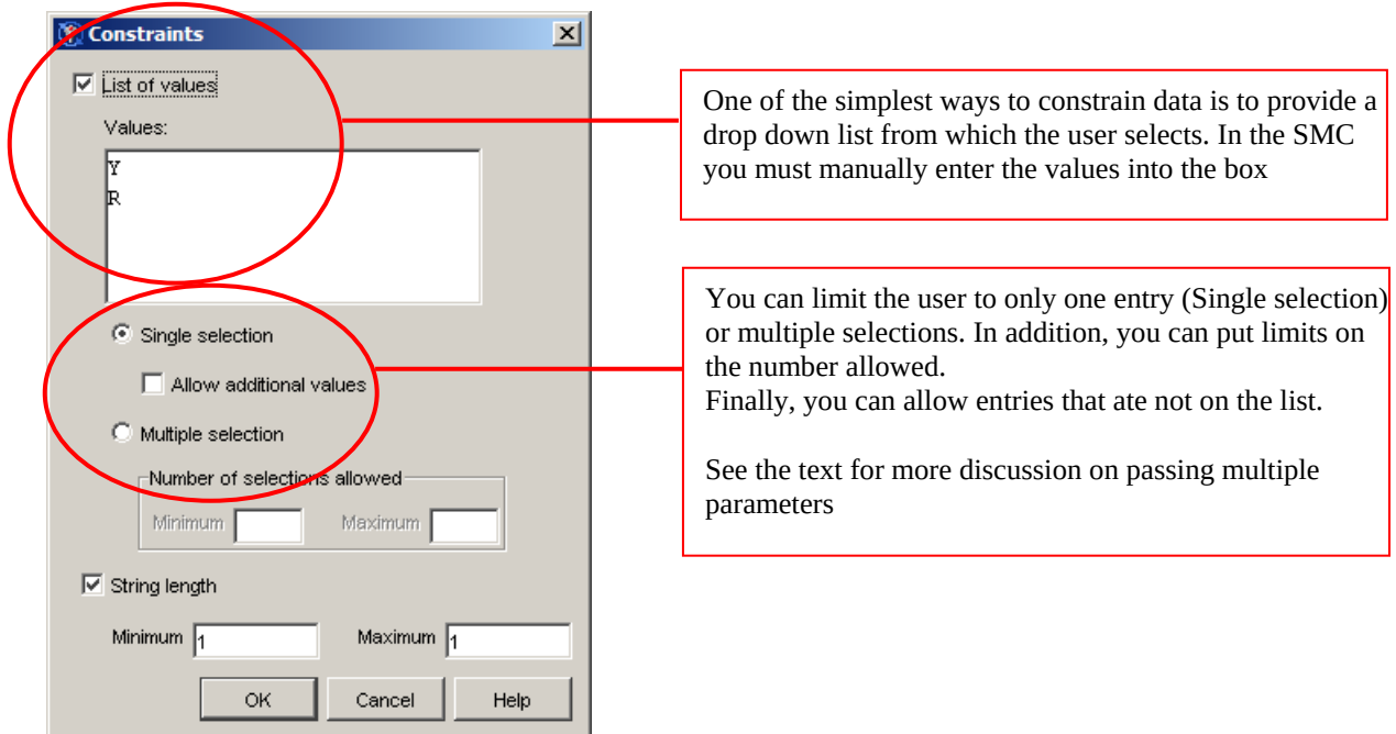
FIGURE 6: PARAMETER CONSTRAINTS
