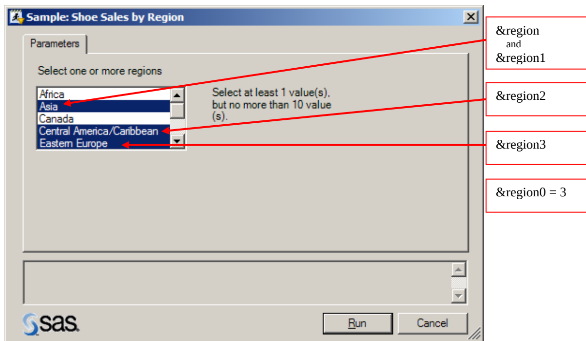
FIGURE 10: SELECTING VALUES
