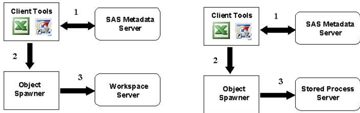
FIGURE 7: EXECUTION FLOW
