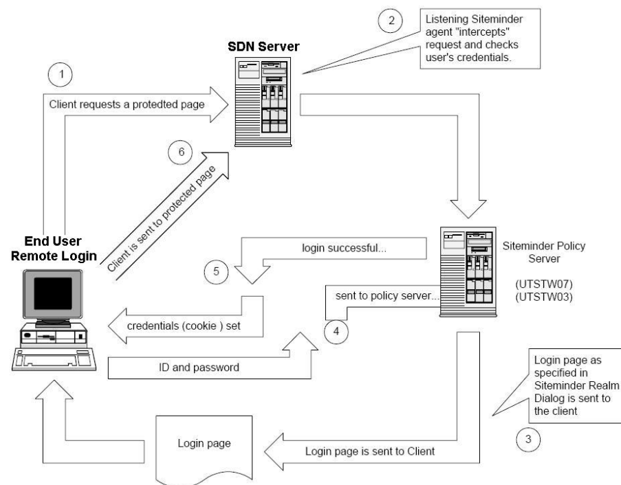
Figure 26 Logical SiteMinder Flow
