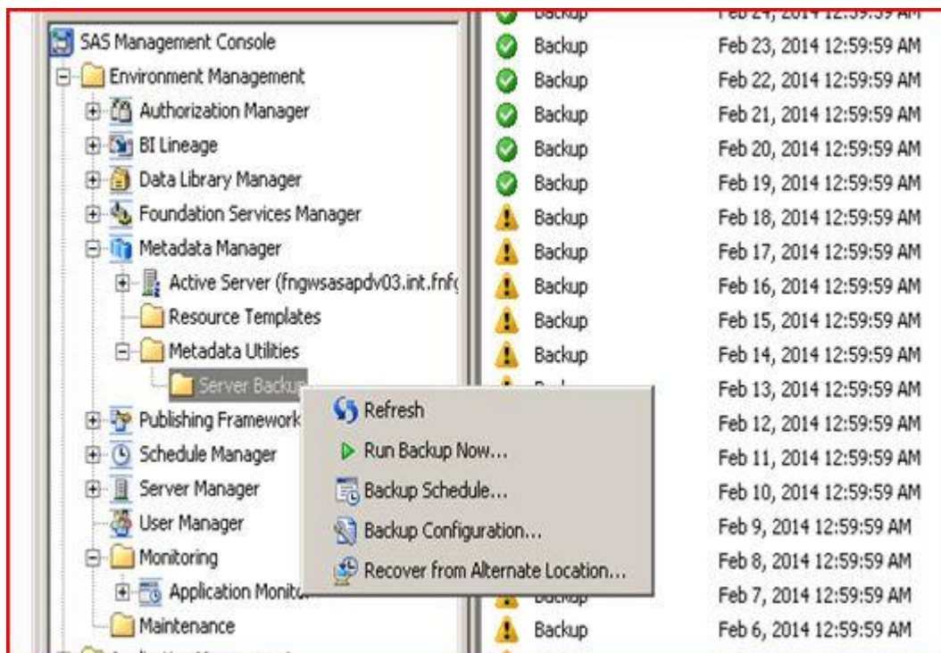
Figure 4. Backup Dialog
