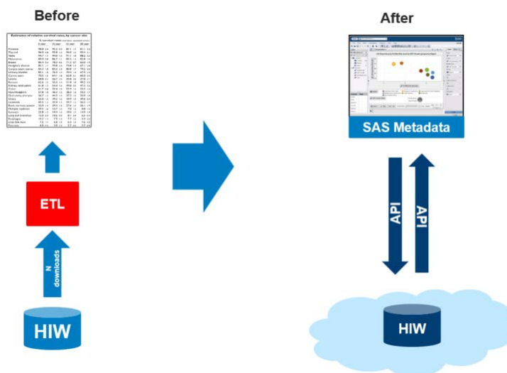
Figure 3. Gap Analysis. Current state (left) without API's and future state (right) with API's reveals the elimination of manual ETL processes (red box) associated with moving data. SAS developers, further, can write stored processes, stored in SAS Metadata, that use the HIW API.
