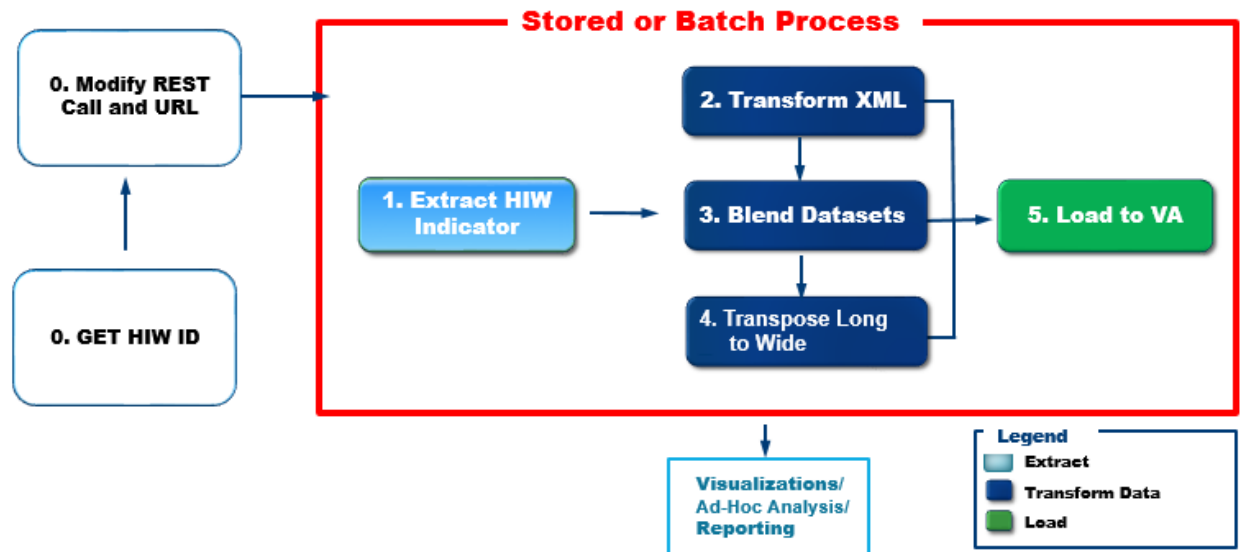
Figure 5. This figure provides a flow chart for the steps involved in accessing HIW data through an API call that loads selected indicators directly into the SAS® Visual Analytics server for analysis.
