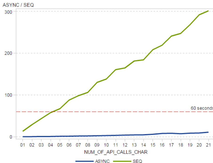
Figure 7. Metrics showing that asynchronous runs of API calls are much faster than sequential runs. The x-axis in the figure shows the number of API calls made by the SAS macro used to extract HIW data, and the y-axis shows the number of seconds they took.
