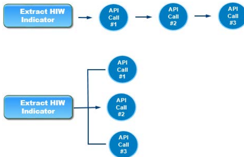
Figure 6. Sequential (top) vs. parallel or asynchronous processing (bottom).
