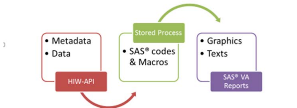
Figure 4. This figure illustrates how organized data such as the data available through the HIW-API service can be used in SAS® Visual Analytics reports by way of stored processes.
