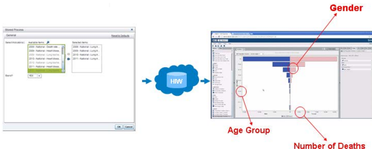
Figure 8. Running a stored process from SAS® Visual Analytics provides immediate access to the HIW data for use in SAS® Visual Analytics visualizations, such as a population pyramid to analyze age groups, gender, and number of deaths. The end-user who downloads a copy of the HIW data may prefer a stored process when response time for data access is short (e.g., less than one minute).
