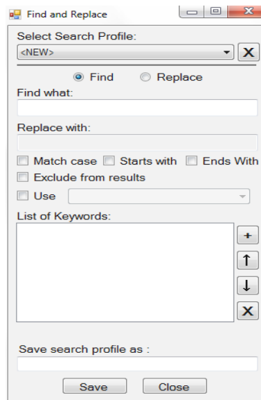
Figure 12. Search Profiler Editor - Find and Replace Dialog Box
