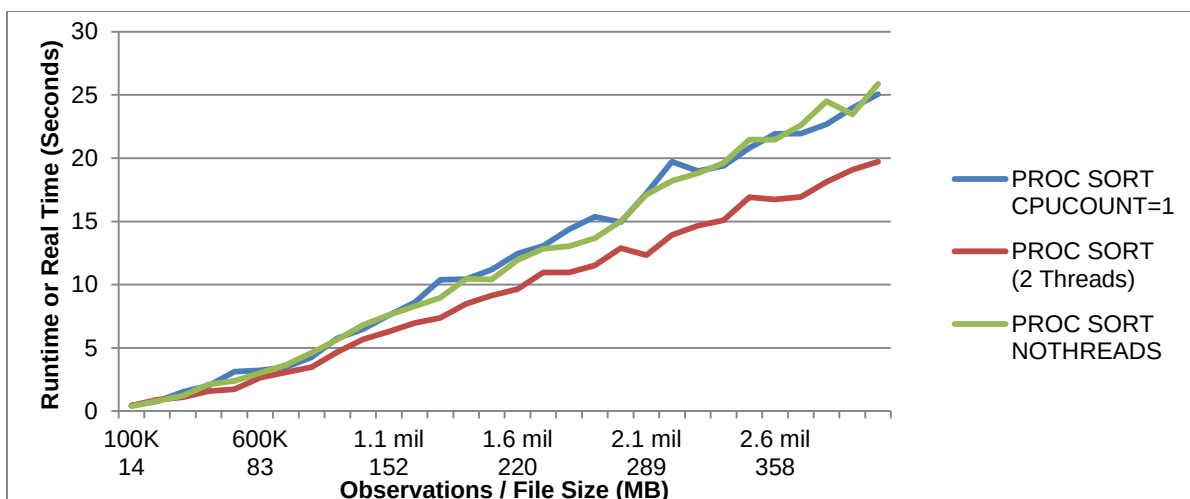
Figure 6. Runtime of SORT Procedure Showing Multithreading Outperforming Single-Threading
