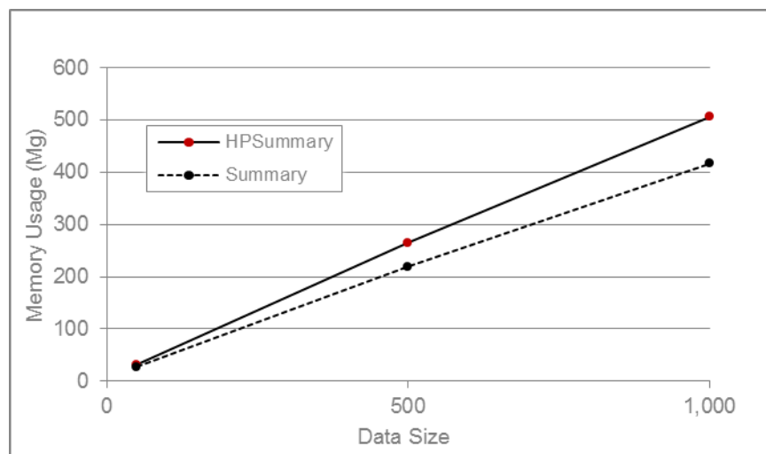
Figure 5: HPSUMMARY and SUMMARY's Memory Usage by Data Size
