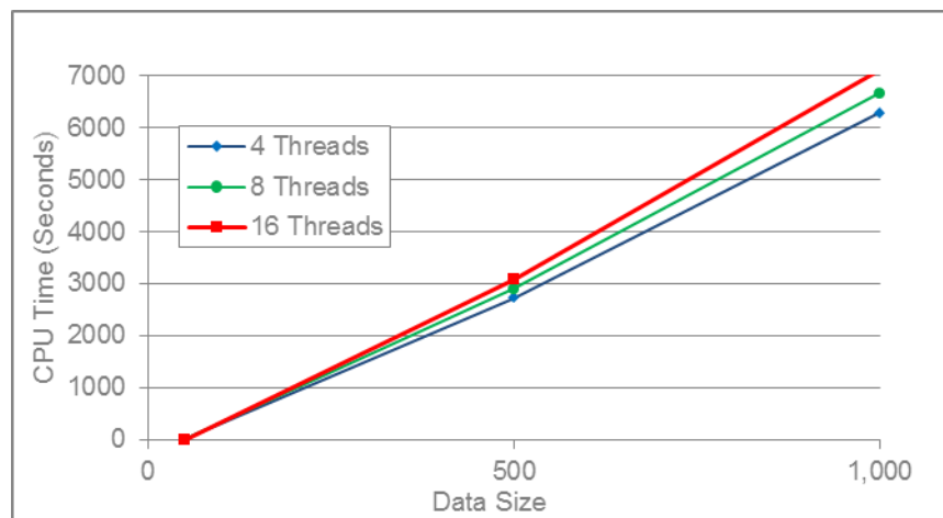
Figure 8: HPSUMMARY's CPU Time for Different Thread Counts
