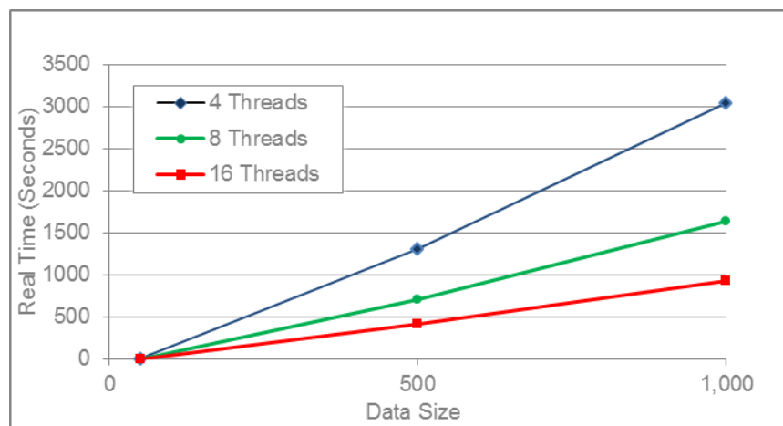
Figure 7: HPSUMMARY's Real Time for Different Thread Counts
