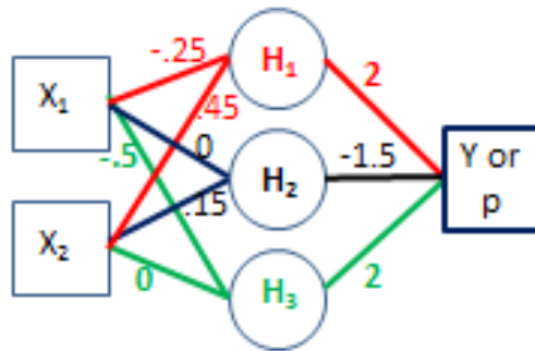
Figure 7. Neural Network Diagram for Figure 8.
