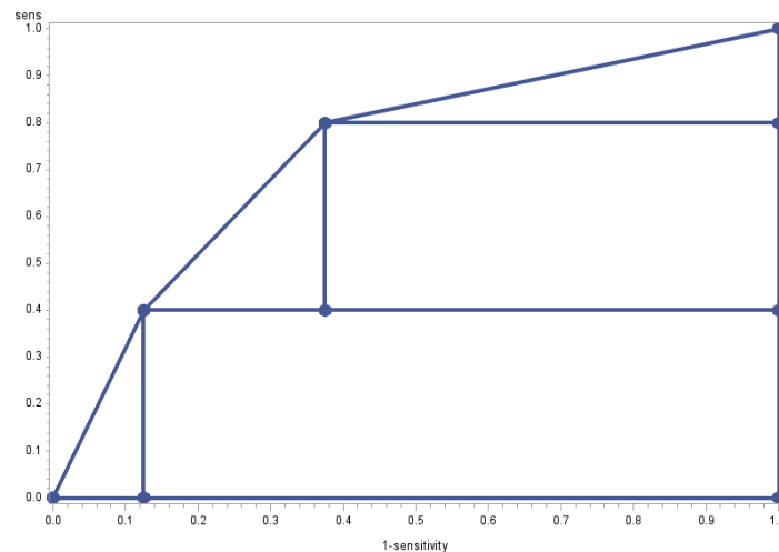
Figure 10. ROC curve for 3 leaf tree.
