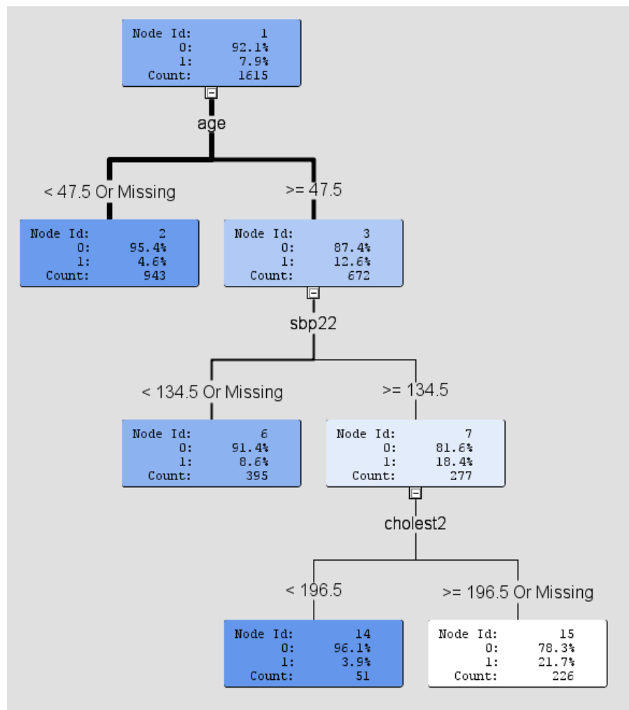
Figure 2. A tree built with SAS Enterprise Miner
