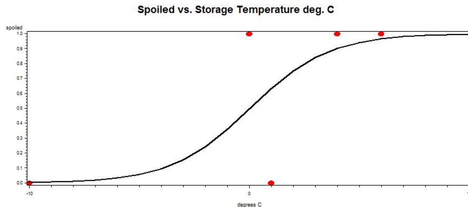
Figure 4. Logistic regression for \Pr\{\text{spoilage}\} versus temperature.
