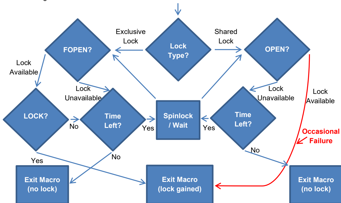
Figure 1. Original (incorrect) %LOCKITDOWN process flow
