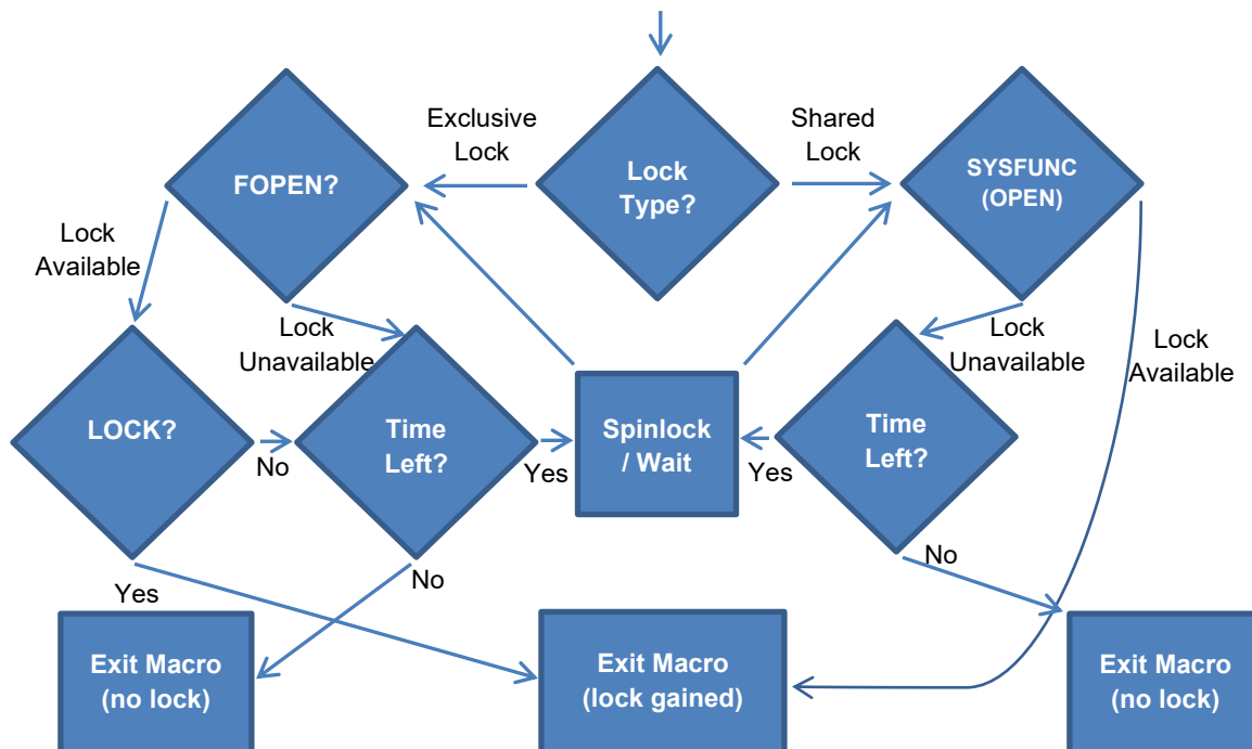
Figure 2. Correct %LOCKITDOWN process flow
