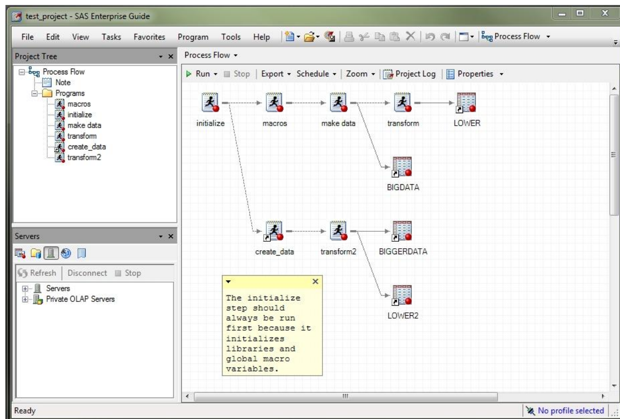
Figure 1. Process Flow View of a SAS Enterprise Guide Project File
