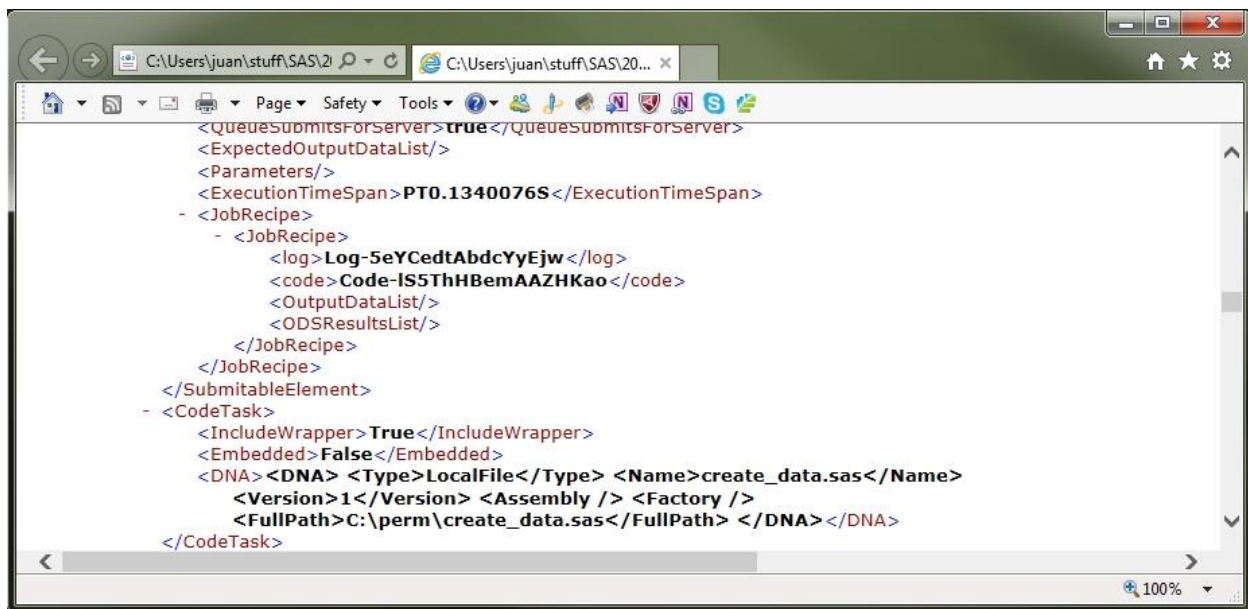
Figure 6. View of a SAS Enterprise Guide Project.xml File (Linked SAS Program)
