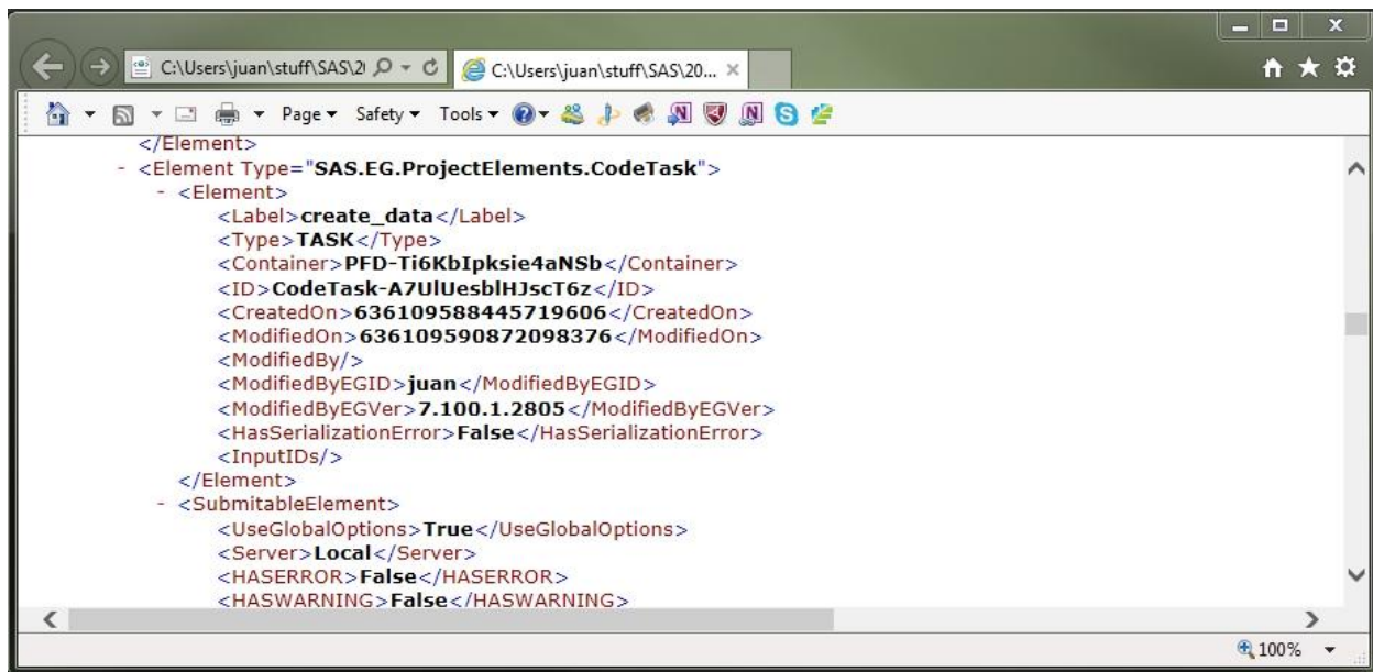
Figure 5. View of a SAS Enterprise Guide Project.xml File (Linked SAS Program)
